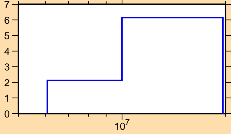
\Delta\sigma/\sigma vs. E for ^{84}\text{As}(n,\text{tot.})
