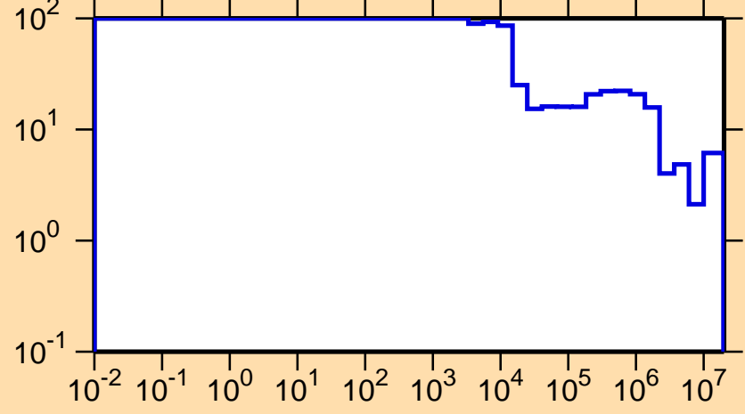
\Delta\sigma/\sigma vs. E for ^{84}\text{As}(n,\text{tot.})
