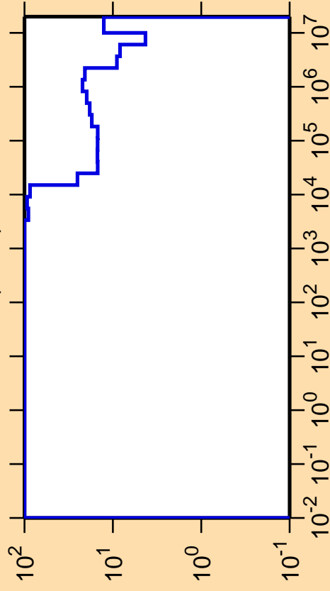
\Delta\sigma/\sigma vs. E for ^{84}\text{As}(n,\text{el.})
