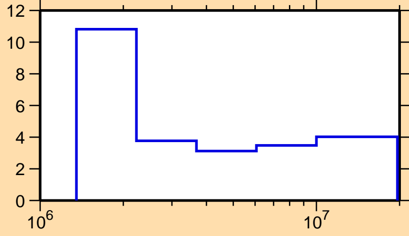
\Delta\sigma/\sigma vs. E for ^{84}\text{As}(n,n\text{onel.})
