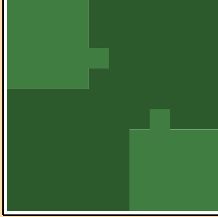
\sigma vs. E for ^{84}\text{As}(n,n_2)
