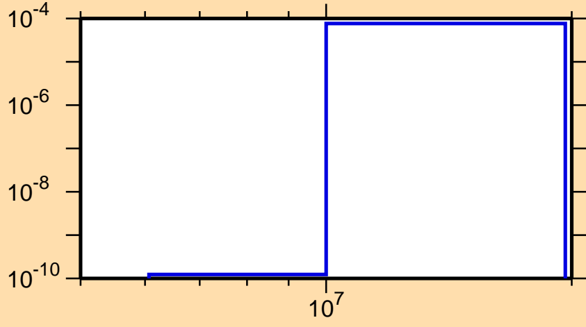
\sigma vs. E for ^{84}\text{As}(n,t)
