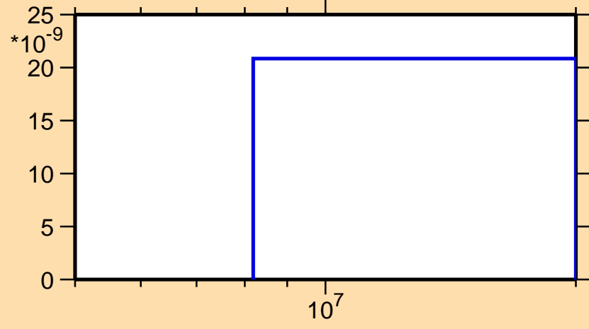
\sigma vs. E for ^{84}\text{As}(n,nt)
