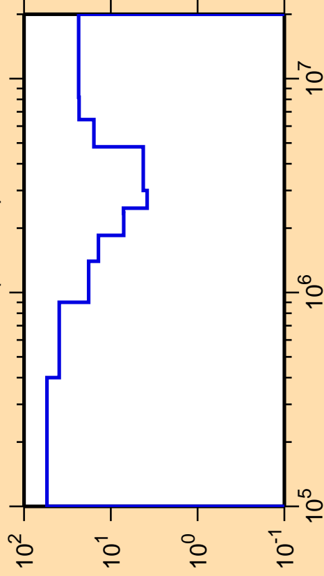
\Delta\sigma/\sigma vs. E for ^{84}\text{As}(n,\text{inel.})
