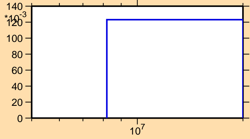
\sigma vs. E for ^{84}\text{As}(n,3n)
