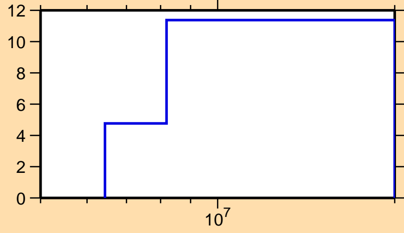
\Delta\sigma/\sigma vs. E for ^{84}\text{As}(n,el.)
