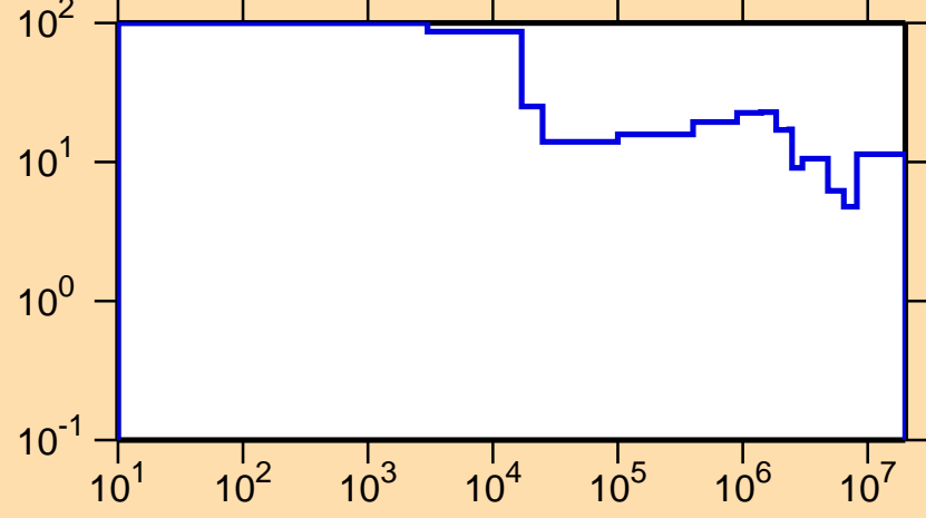
\Delta\sigma/\sigma vs. E for ^{84}\text{As}(n,\text{el.})
