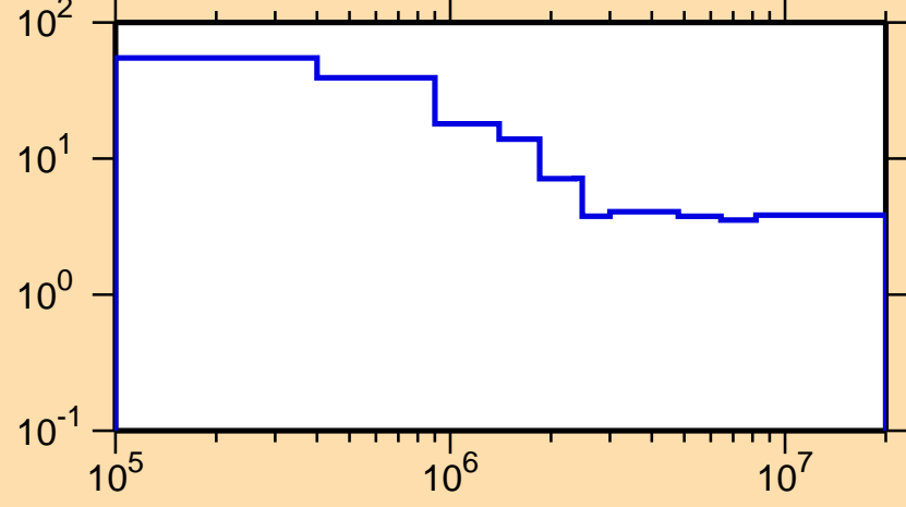
\Delta\sigma/\sigma vs. E for ^{84}\text{As}(n,\text{nonel.})
