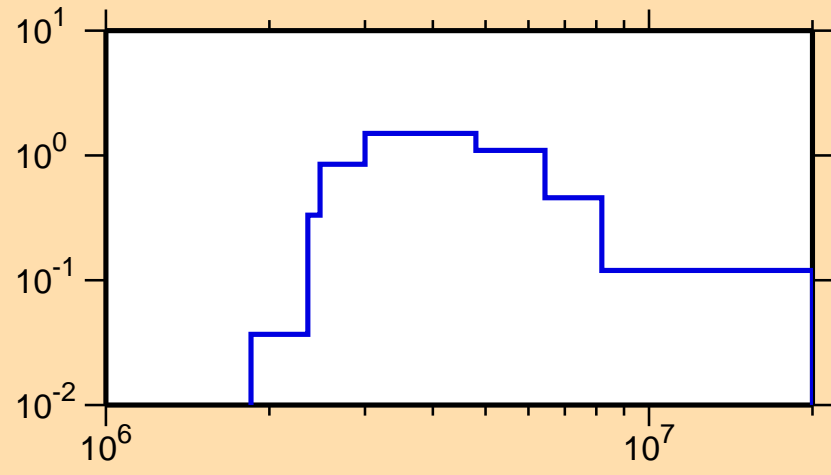
\sigma vs. E for ^{84}\text{As}(n,n\text{cont.})
