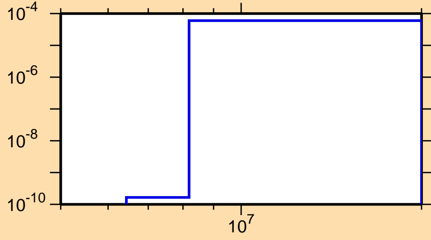
\sigma vs. E for ^{84}\text{As}(n,\alpha)
