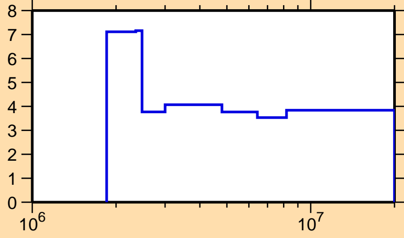
\Delta\sigma/\sigma vs. E for ^{84}\text{As}(n,n\text{onel.})
