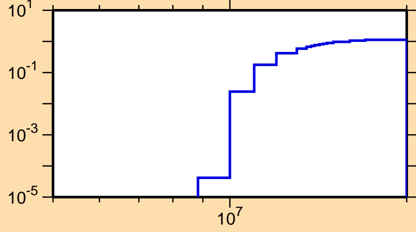
\sigma vs. E for ^{85}\text{As}(n,3n)
