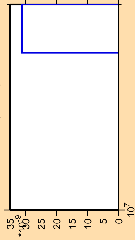
\Delta\sigma/\sigma vs. E for ^{85}\text{As} (mt 11)
