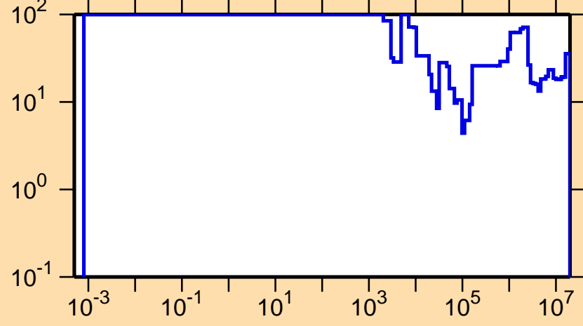
\Delta\sigma/\sigma vs. E for ^{85}\text{As}(n,\text{el.})
