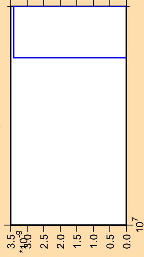
\Delta\sigma/\sigma vs. E for ^{85}\text{As}(n,3n\alpha)
