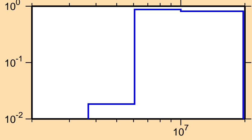
\sigma vs. E for ^{85}\text{As}(n,2n)
