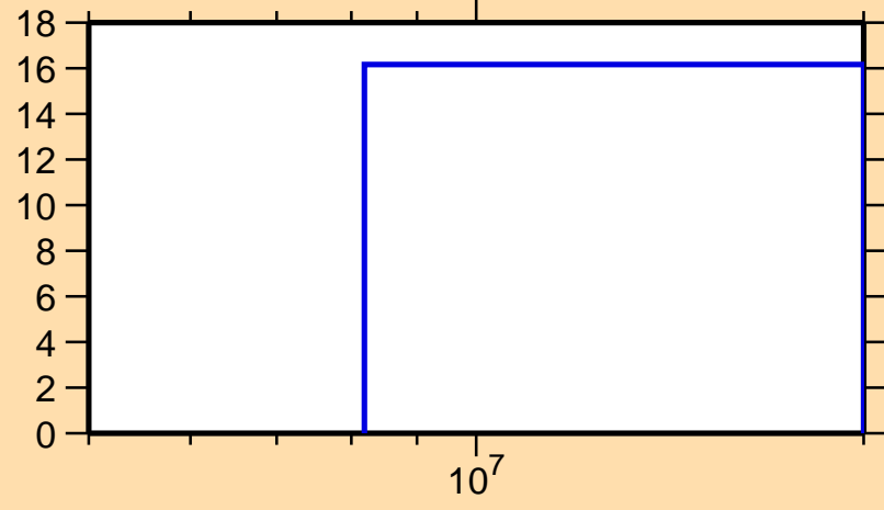
\Delta\sigma/\sigma vs. E for ^{85}\text{As}(n,el.)
