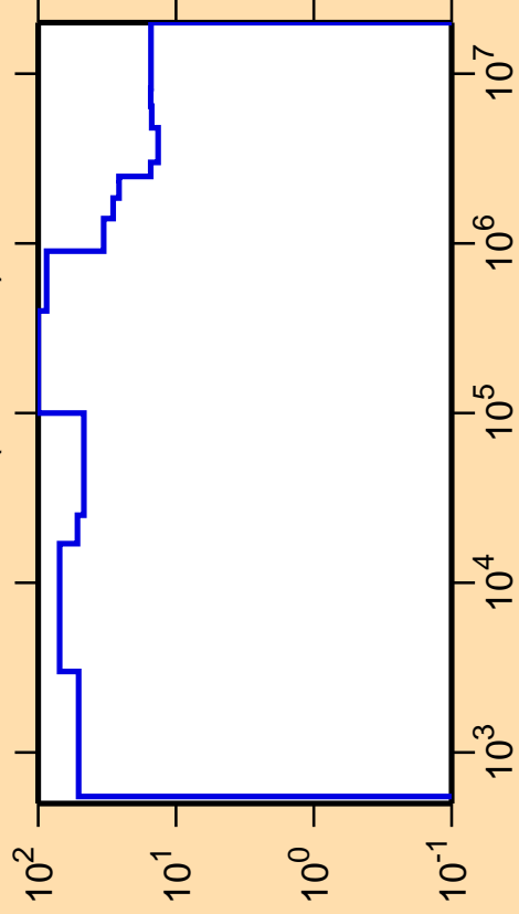
\Delta\sigma/\sigma vs. E for ^{85}\text{As}(n,\text{nonel.})
