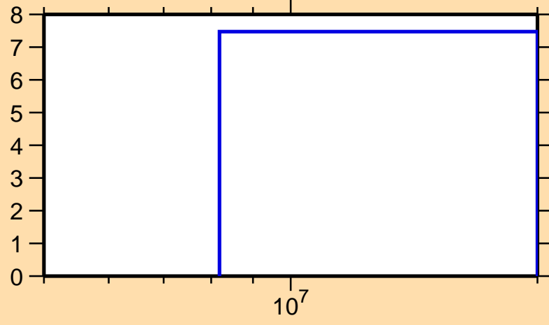
\Delta\sigma/\sigma vs. E for ^{85}\text{As}(n,\text{tot.})
