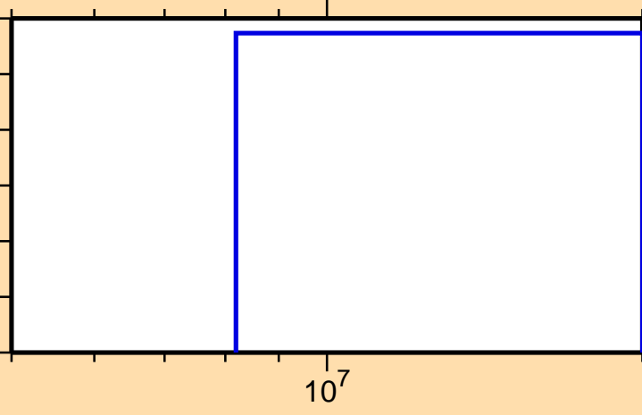
\sigma vs. E for ^{85}\text{As}(n,d)
