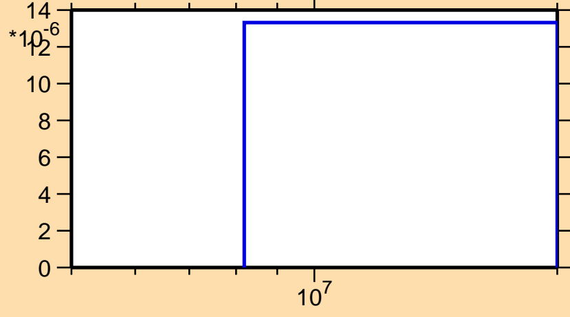
\sigma vs. E for ^{85}\text{As}(n,t)
