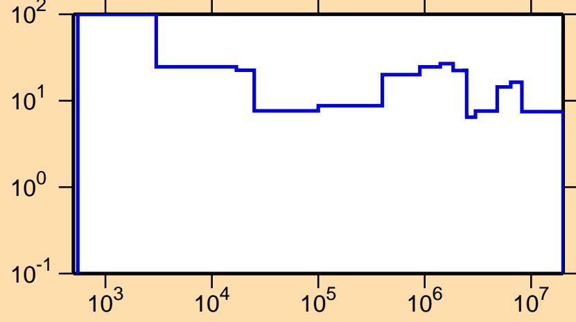
\Delta\sigma/\sigma vs. E for ^{85}\text{As}(n,\text{tot.})
