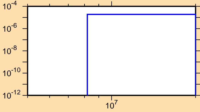
\sigma vs. E for ^{85}\text{As}(n,\alpha)
