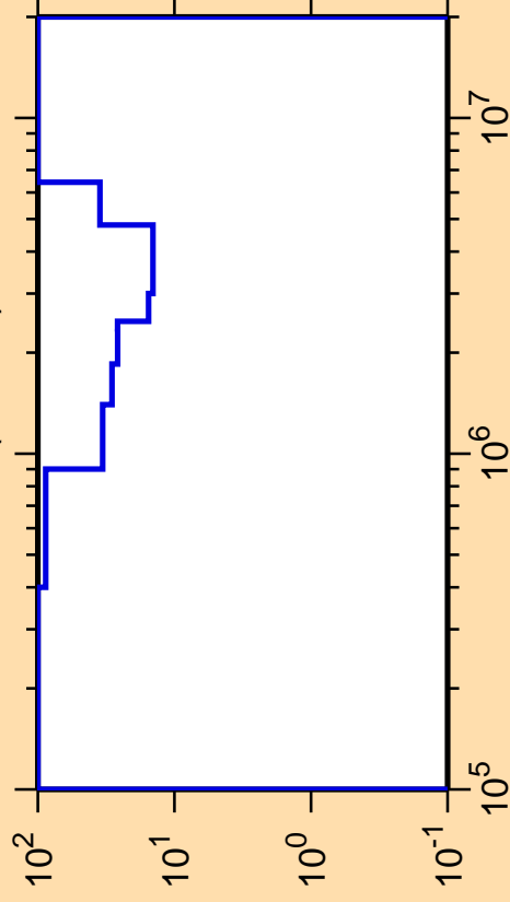
\Delta\sigma/\sigma vs. E for ^{85}\text{As}(n,\text{inel.})
