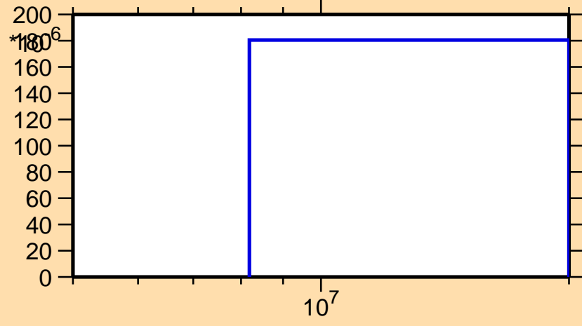
\sigma vs. E for ^{85}\text{As}(n,p)
