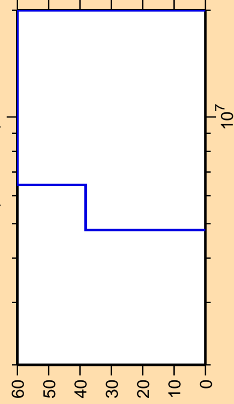
\Delta\sigma/\sigma vs. E for ^{85}\text{As}(n,n\text{cont.})
