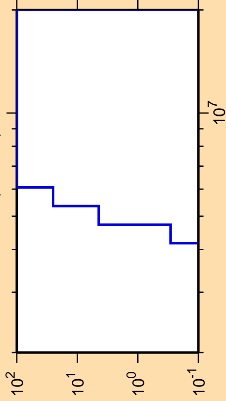
\Delta\sigma/\sigma vs. E for ^{197}\text{At}(\text{mt117})
