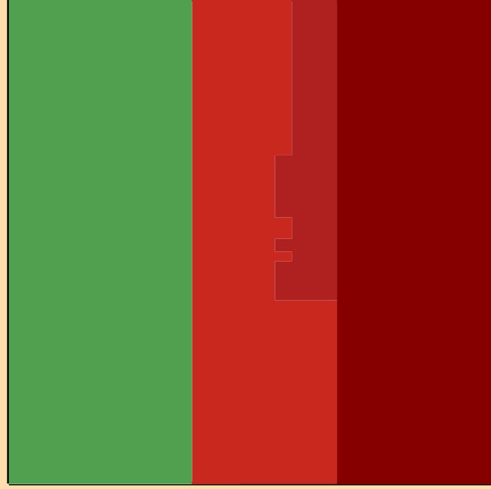
\Delta\sigma/\sigma vs. E for ^{197}\text{At}(n,2n)
