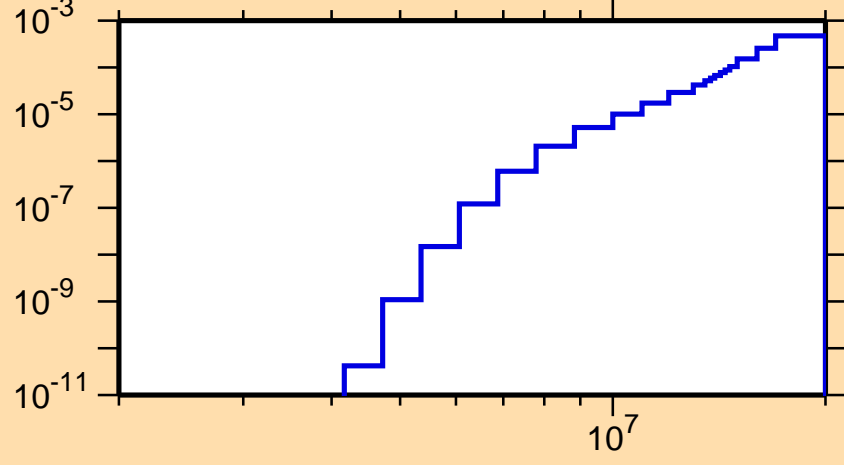
\sigma vs. E for ^{197}\text{At}(\text{mt } 45)
