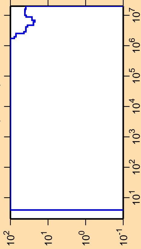
\Delta\sigma/\sigma vs. E for ^{197}\text{At}(n,\text{inel.})
