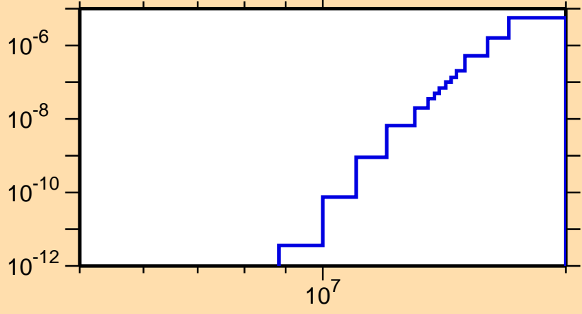
\sigma vs. E for ^{197}\text{At}(n,pd)
