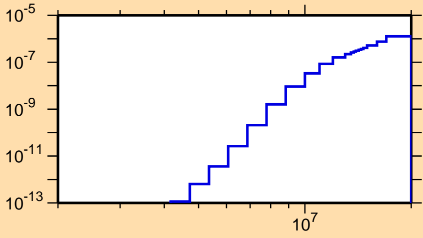
\sigma vs. E for ^{197}\text{At}(\text{mt117})
