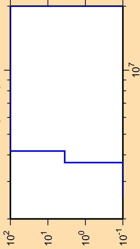
\Delta\sigma/\sigma vs. E for ^{197}\text{At}(\text{mt } 45)
