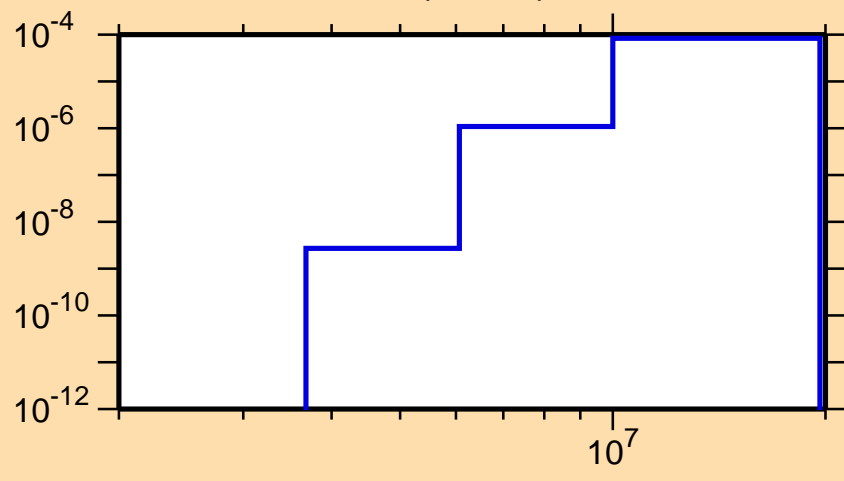
\sigma vs. E for ^{197}\text{At}(\text{mt } 45)
