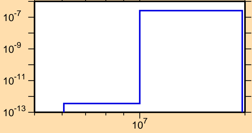
\sigma vs. E for ^{197}\text{At}(n,\text{pd})
