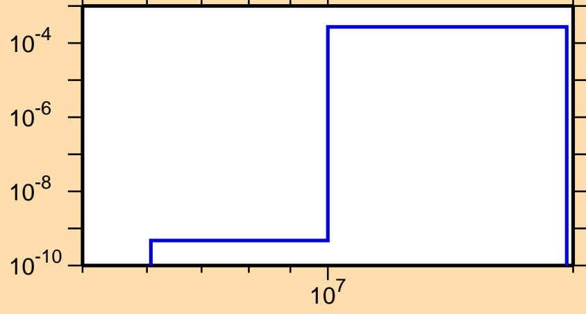
\sigma vs. E for ^{197}\text{At}(n,t)
