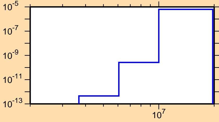
\sigma vs. E for ^{197}\text{At}(n,\text{He}3)
