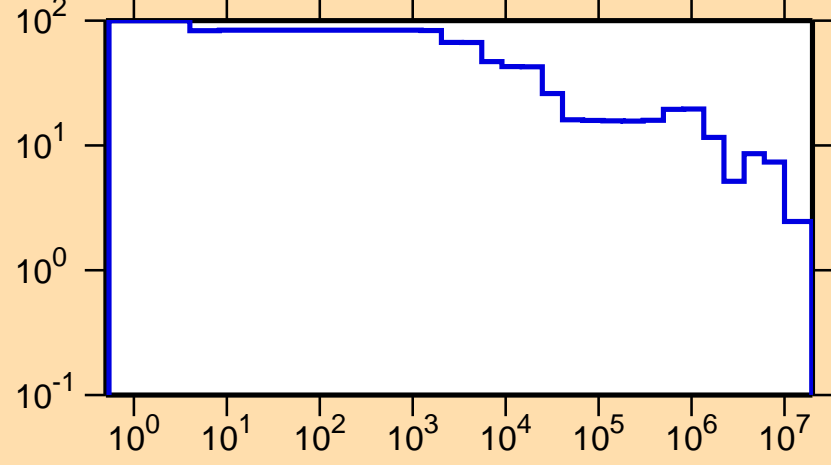
\Delta\sigma/\sigma vs. E for ^{197}\text{At}(n,\text{tot.})
