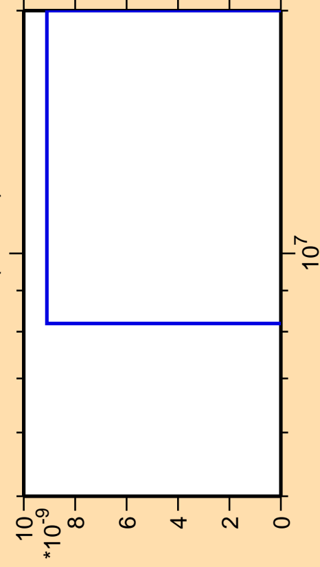
\Delta\sigma/\sigma vs. E for ^{197}\text{At}(\text{mt } 42)
