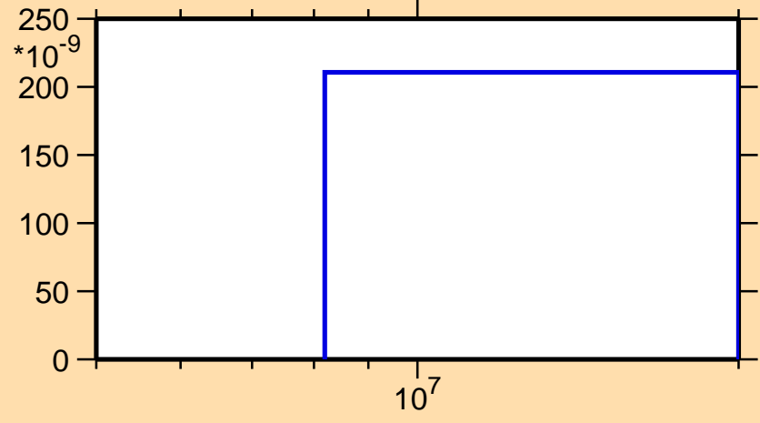
\sigma vs. E for ^{197}\text{At}(n,\text{pd})
