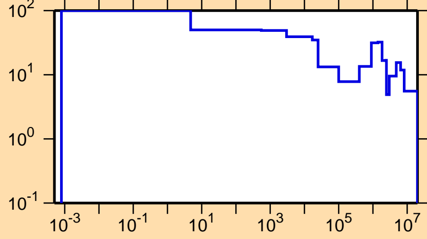
\Delta\sigma/\sigma vs. E for ^{197}\text{At}(n,\text{el.})
