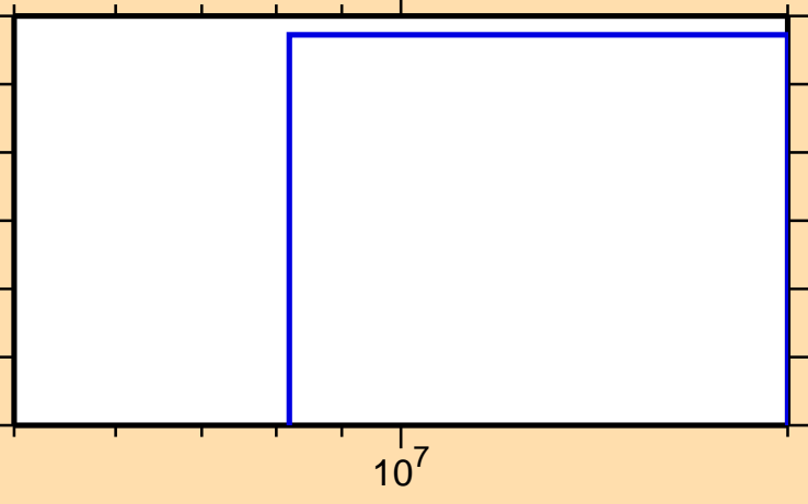
\sigma vs. E for ^{197}\text{At}(n,\text{pt})
