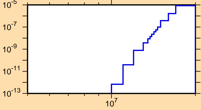
\sigma vs. E for ^{198}\text{At}(n,\text{nd})
