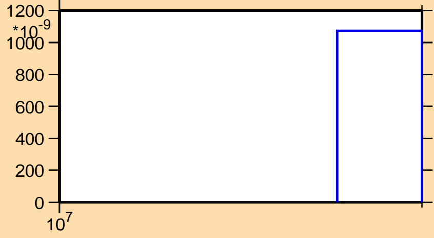
\sigma vs. E for ^{198}\text{At}(n,3n)
