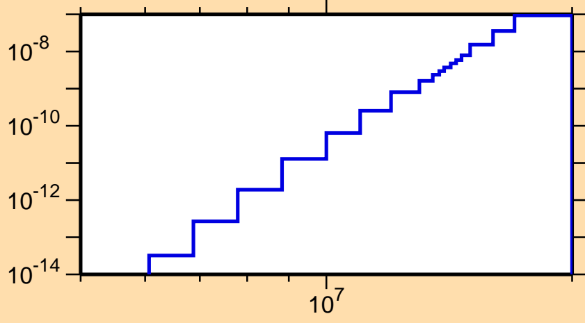
\sigma vs. E for ^{198}\text{At}(\text{mt117})
