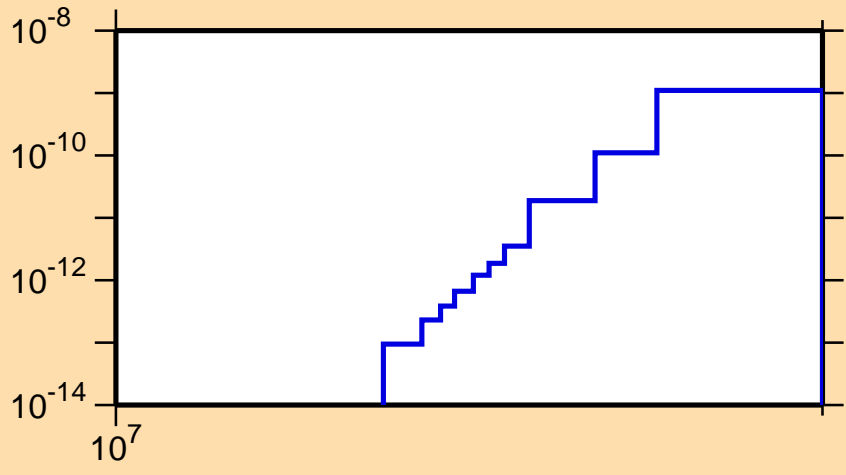
\sigma vs. E for ^{198}\text{At}(\text{mt } 34)
