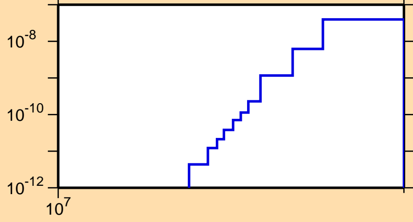
\sigma vs. E for ^{198}\text{At}(n,pt)
