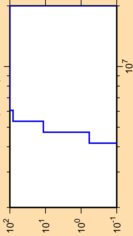
\Delta\sigma/\sigma vs. E for ^{198}\text{At}(n,\text{He}3)
