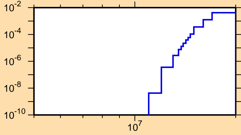
\sigma vs. E for ^{198}\text{At}(n,2np)
