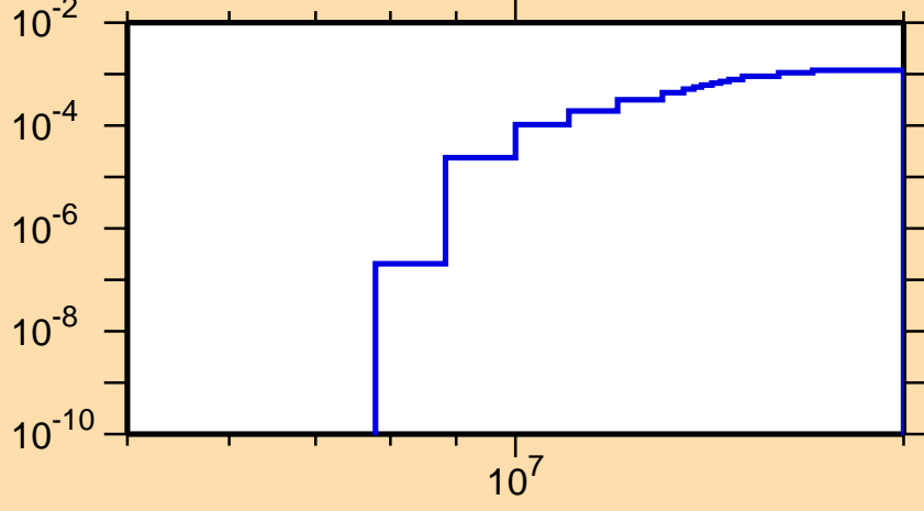
\sigma vs. E for ^{198}\text{At}(n,2n\alpha)
