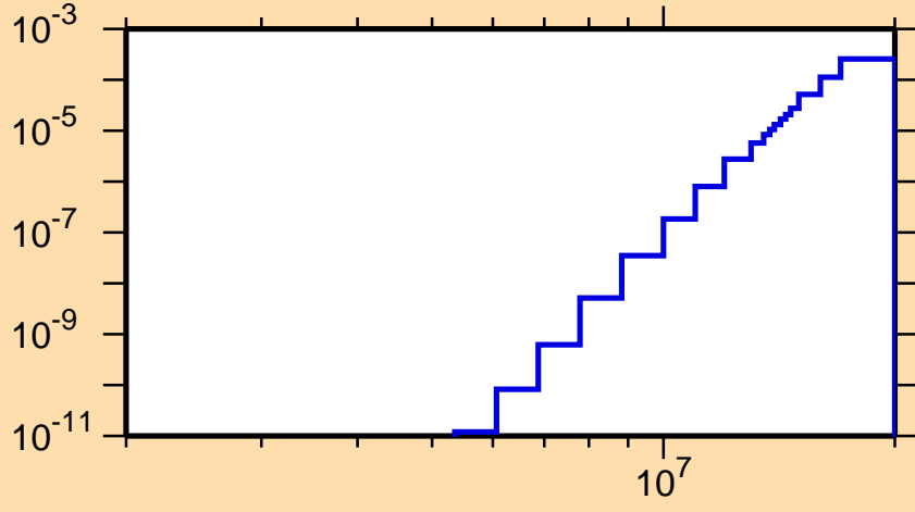
\sigma vs. E for ^{198}\text{At}(n,\text{He}3)
