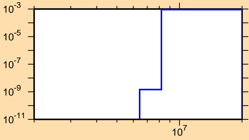
\sigma vs. E for ^{198}\text{At}(n,t)
