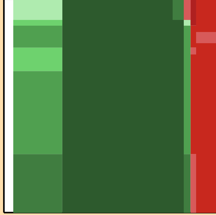
\Delta\sigma/\sigma vs. E for ^{198}\text{At}(n,n\text{cont.})
