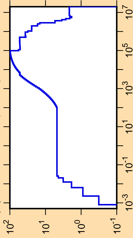
\Delta\mu/\mu vs. E for ^{199}\text{At}(\text{mt251})
