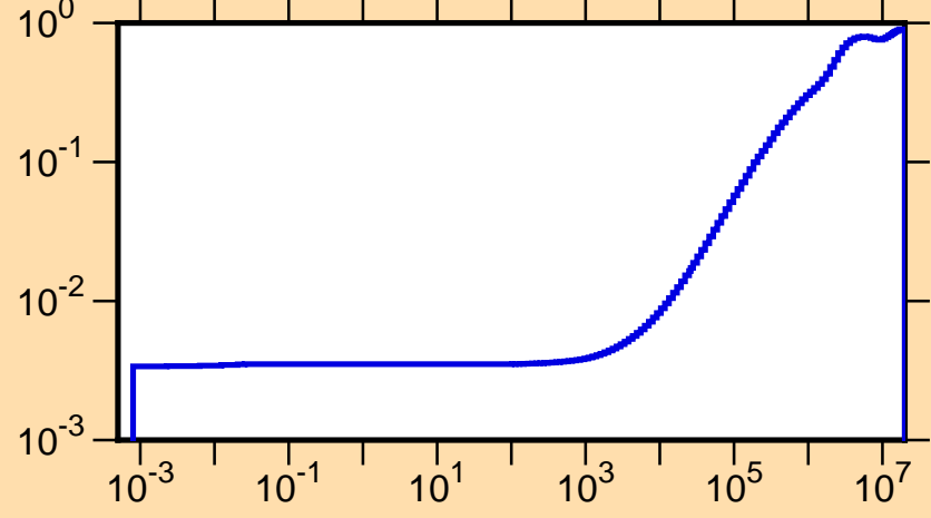
\mu vs. E for ^{199}\text{At}(\text{mt251})
