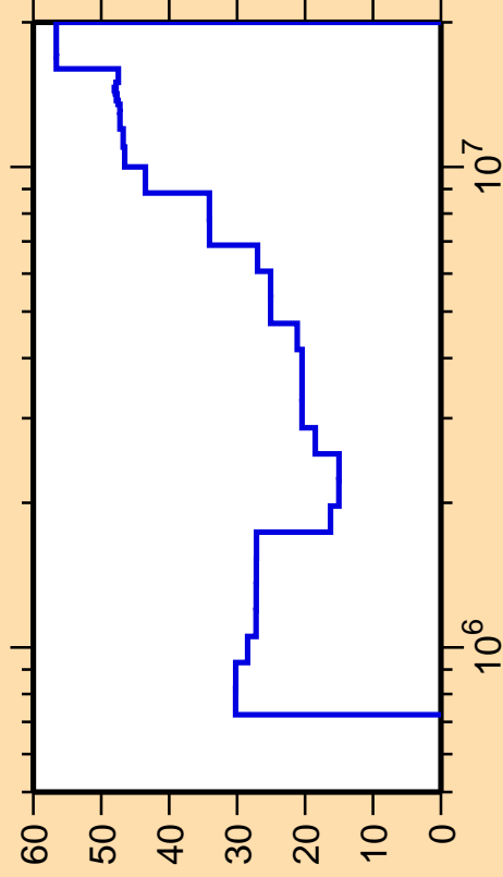
\Delta\sigma/\sigma vs. E for ^{199}\text{At}(n,\gamma)
