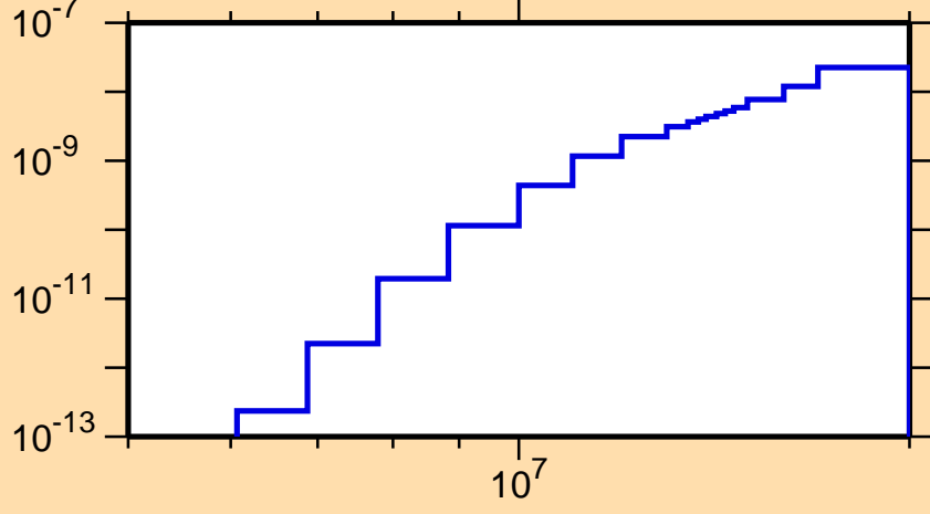
\sigma vs. E for ^{199}\text{At}(\text{mt117})
