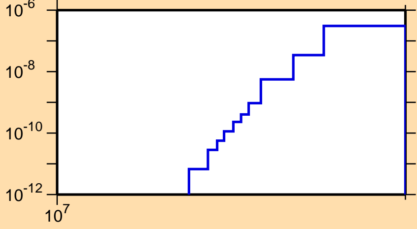
\sigma vs. E for ^{199}\text{At}(n,nd)
