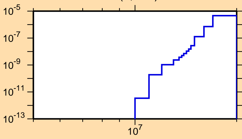
\sigma vs. E for ^{199}\text{At}(n,2n\alpha)
