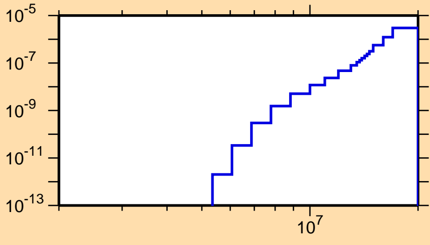
\sigma vs. E for ^{199}\text{At}(\text{mt } 45)
