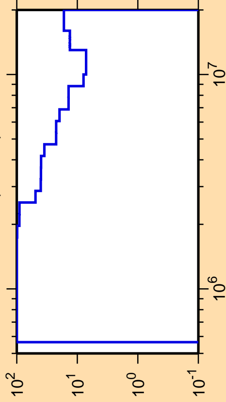
\Delta\sigma/\sigma vs. E for ^{199}\text{At}(n,\text{inel.})
