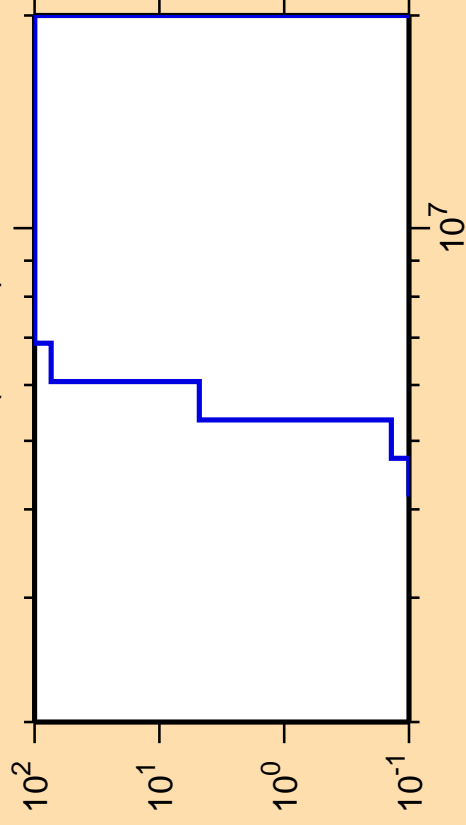
\Delta\sigma/\sigma vs. E for ^{199}\text{At}(\text{mt } 45)
