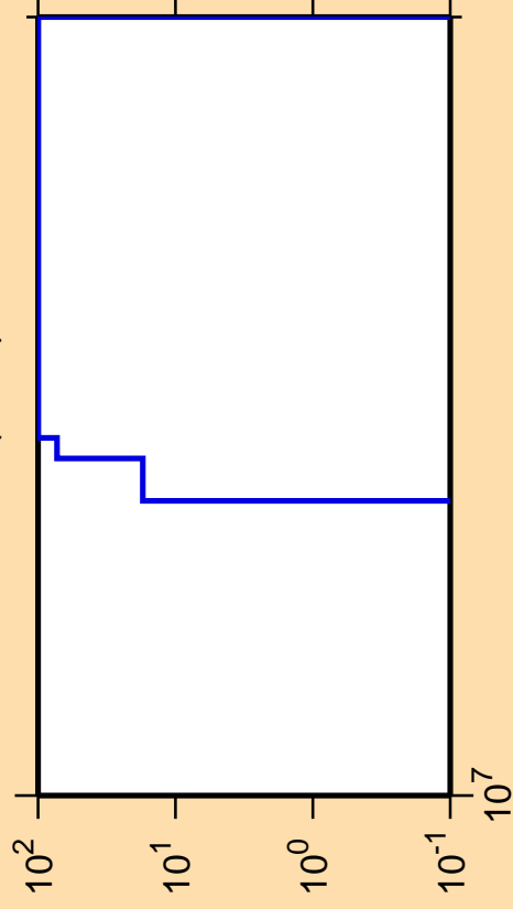
\Delta\sigma/\sigma vs. E for ^{199}\text{At}(n,nd)
