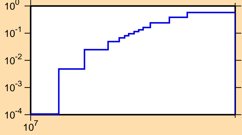
\sigma vs. E for ^{199}\text{At}(n,2n)
