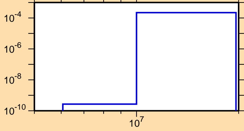
\sigma vs. E for ^{199}\text{At}(n,t)
