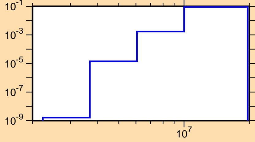
\sigma vs. E for ^{199}\text{At}(n,np)
