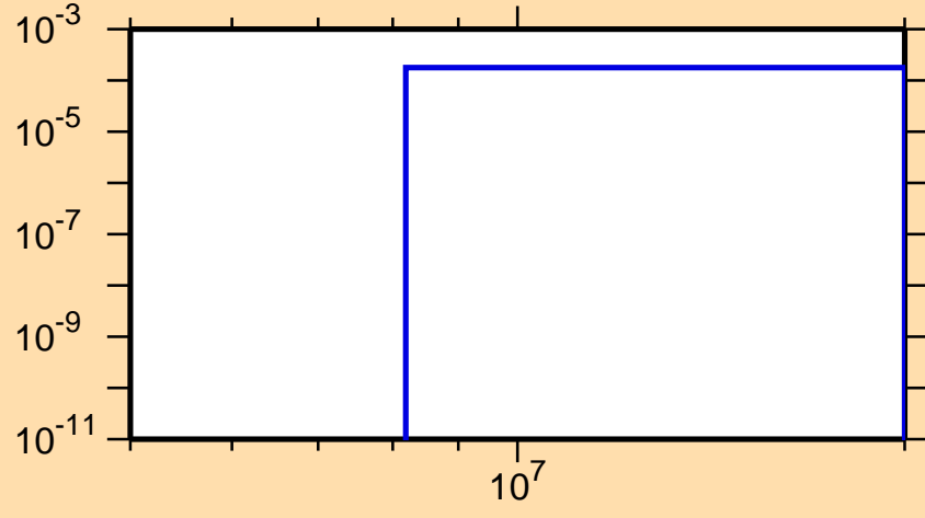
\sigma vs. E for ^{199}\text{At}(n,t)
