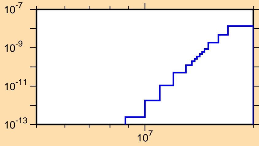
\sigma vs. E for ^{200}\text{At}(\text{mt117})
