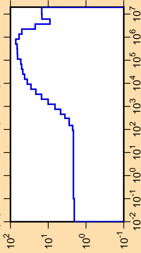
\Delta\mu/\mu vs. E for ^{200}\text{At}(\text{mt251})
