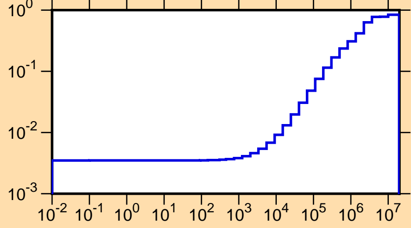
\mu vs. E for ^{200}\text{At}(\text{mt251})
