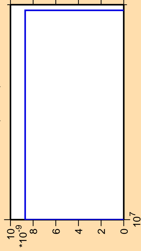
\Delta\sigma/\sigma vs. E for ^{200}\text{At}(\text{mt } 42)
