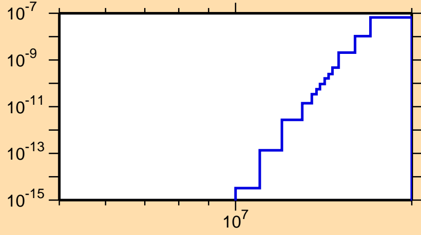
\sigma vs. E for ^{200}\text{At}(n,pd)
