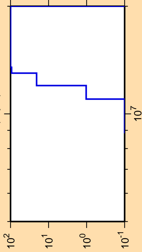
\Delta\sigma/\sigma vs. E for ^{200}\text{At}(n,pd)
