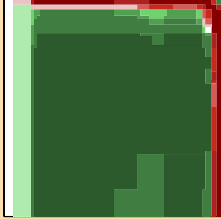
\Delta\sigma/\sigma vs. E for ^{200}\text{At}(n,n\text{cont.})
