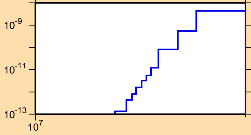
\sigma vs. E for ^{200}\text{At}(n,pt)
