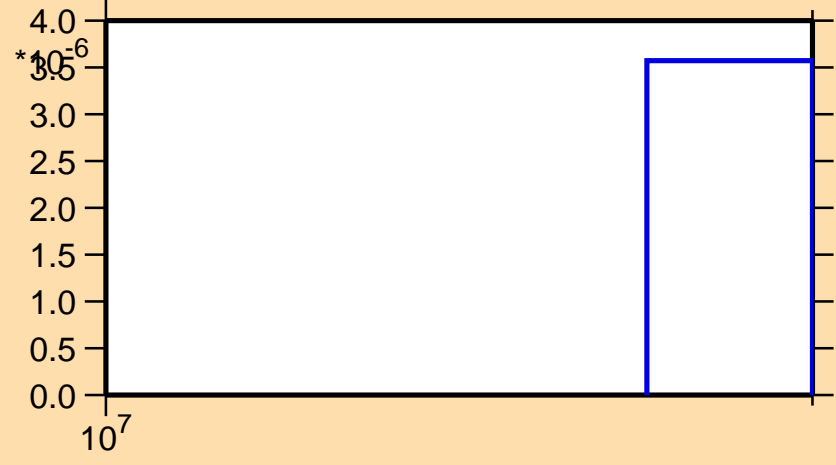
\sigma vs. E for ^{200}\text{At}(n,3n)
