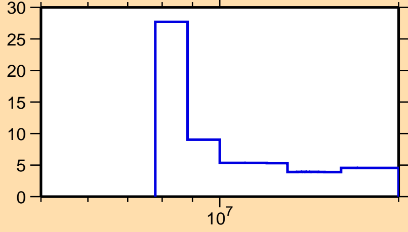
\Delta\sigma/\sigma vs. E for ^{200}\text{At}(n,\text{el.})
