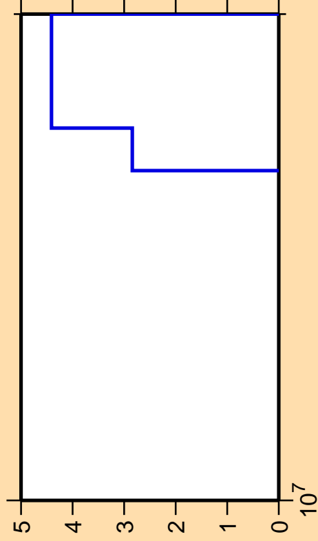
\Delta\sigma/\sigma vs. E for ^{200}\text{At}(n,3n\alpha)
