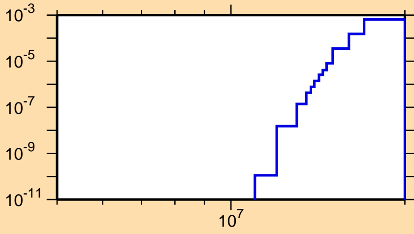
\sigma vs. E for ^{200}\text{At}(n,2np)
