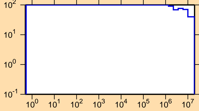
\Delta\sigma/\sigma vs. E for ^{200}\text{At}(n,n_1)
