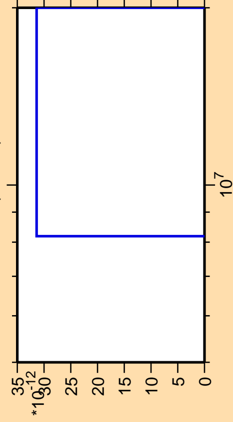
\Delta\sigma/\sigma vs. E for ^{200}\text{At}(\text{mt } 42)
