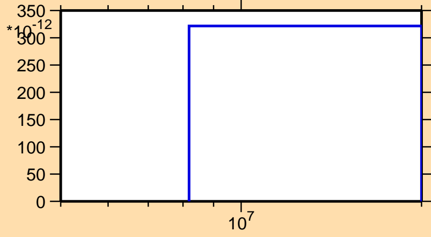
\sigma vs. E for ^{200}\text{At}(\text{mt117})
