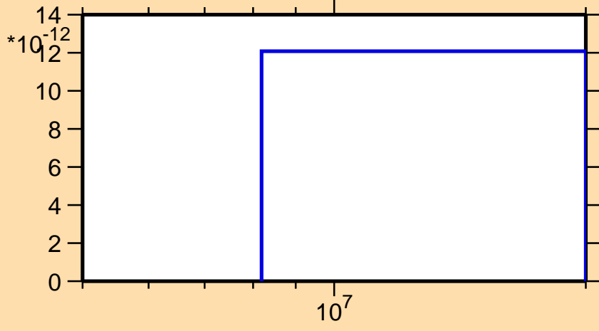
\sigma vs. E for ^{200}\text{At}(n,nt)
