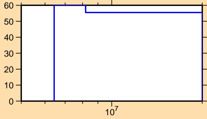
\Delta\sigma/\sigma vs. E for ^{200}\text{At}(n,2n)
