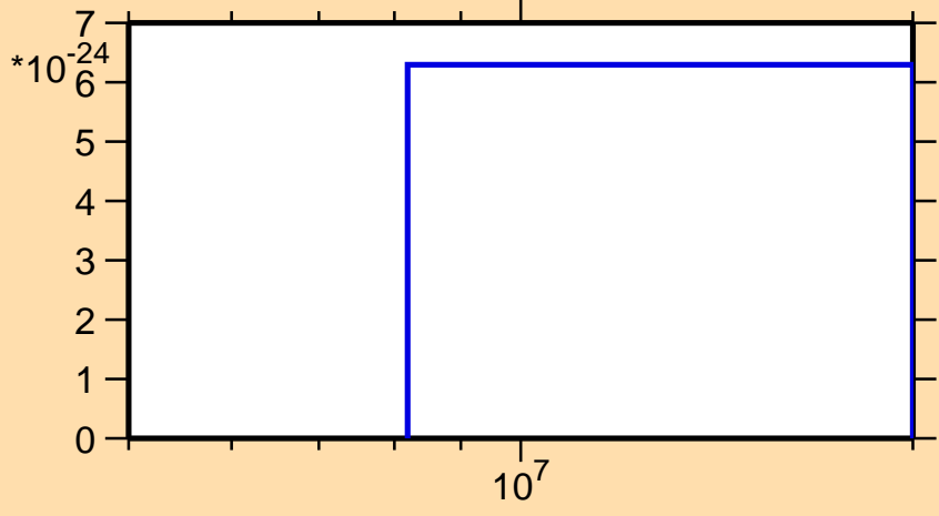
\sigma vs. E for ^{200}\text{At}(\text{mt } 42)
