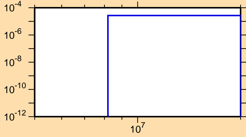
\sigma vs. E for ^{200}\text{At}(n,2n\alpha)
