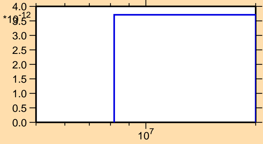
\sigma vs. E for ^{200}\text{At}(\text{mt } 34)
