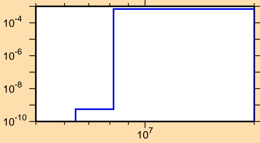
\sigma vs. E for ^{200}\text{At}(n,t)
