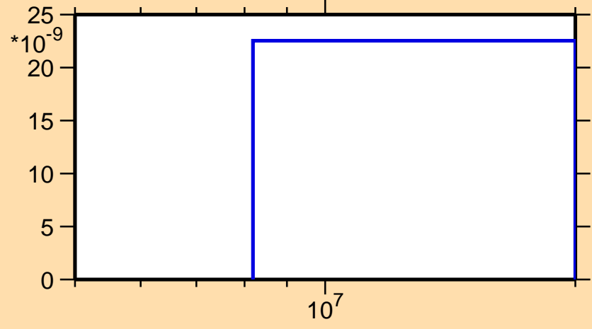
\sigma vs. E for ^{200}\text{At}(\text{mt } 45)
