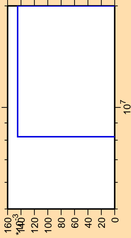
\Delta\sigma/\sigma vs. E for ^{200}\text{At}(n,3n\alpha)
