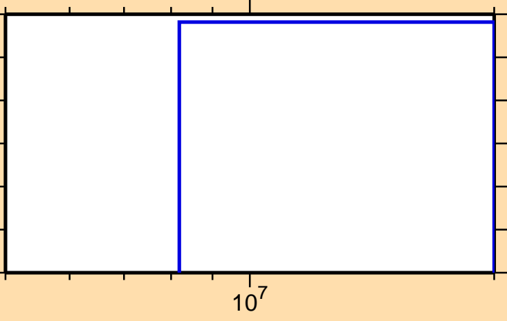
\sigma vs. E for ^{200}\text{At}(n,3n)
