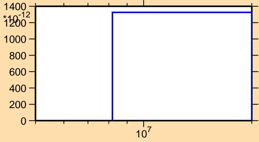
\sigma vs. E for ^{200}\text{At}(n,\text{pd})
