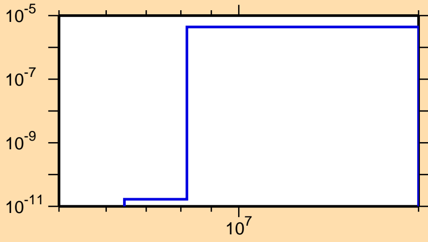
\sigma vs. E for ^{200}\text{At}(n,\text{He}3)
