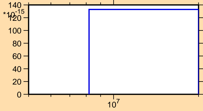
\sigma vs. E for ^{200}\text{At}(n,3n\alpha)
