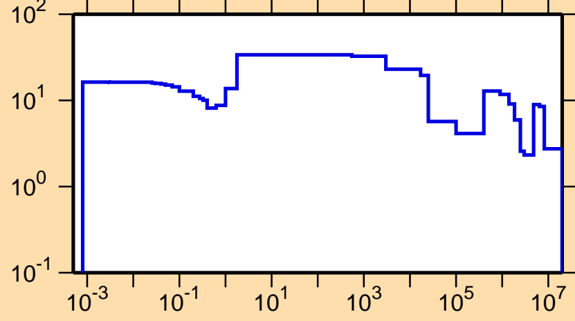
\Delta\sigma/\sigma vs. E for ^{200}\text{At}(n,\text{tot.})
