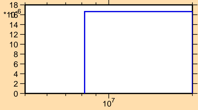
\sigma vs. E for ^{200}\text{At}(n,2np)
