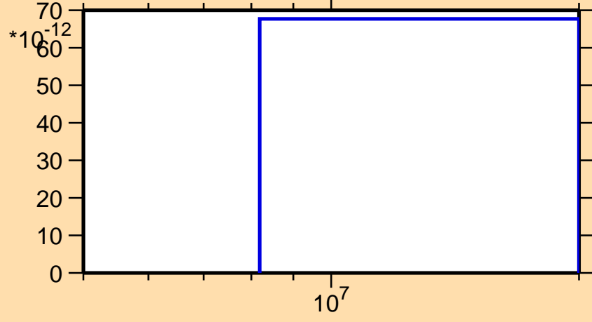
\sigma vs. E for ^{200}\text{At}(n,\text{pt})
