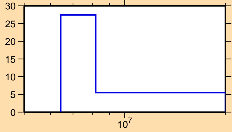
\Delta\sigma/\sigma vs. E for ^{200}\text{At}(n,el.)
