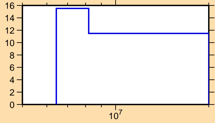
\Delta\sigma/\sigma vs. E for ^{200}\text{At}(n,\text{nonel.})
