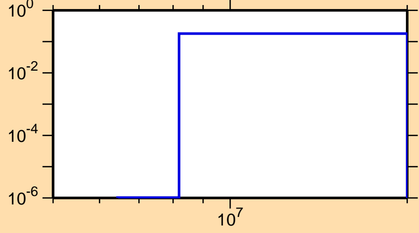
\sigma vs. E for ^{200}\text{At}(n,2n)
