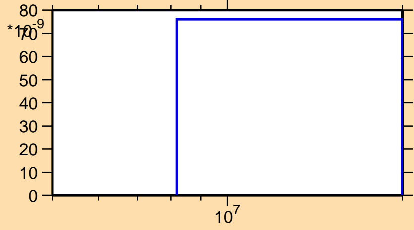
\sigma vs. E for ^{200}\text{At}(n,\text{nd})
