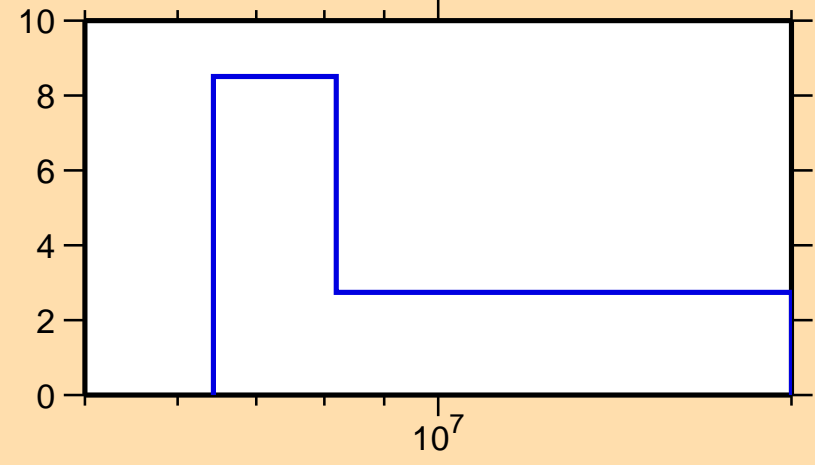
\Delta\sigma/\sigma vs. E for ^{200}\text{At}(n,\text{tot.})
