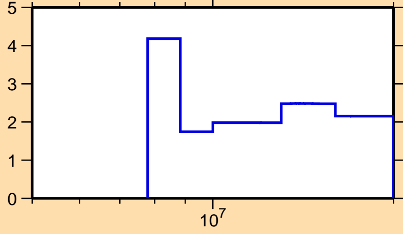
\Delta\sigma/\sigma vs. E for ^{202}\text{At}(n,\text{el.})
