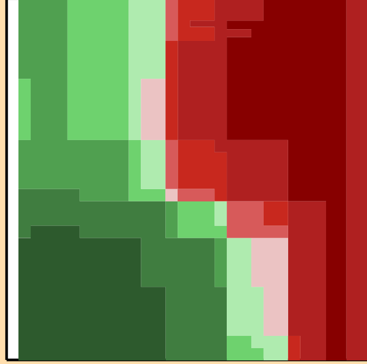
\Delta\sigma/\sigma vs. E for ^{202}\text{At}(n,n\text{cont.})
