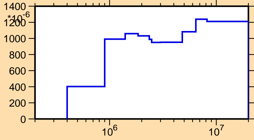
\sigma vs. E for ^{202}\text{At}(n,n_4)
