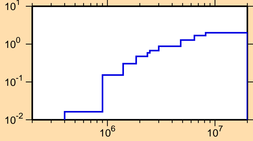
\sigma vs. E for ^{202}\text{At}(n,\text{inel.})
