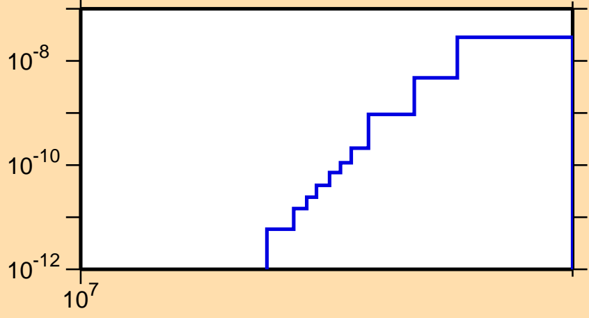
\sigma vs. E for ^{202}\text{At}(n,pd)
