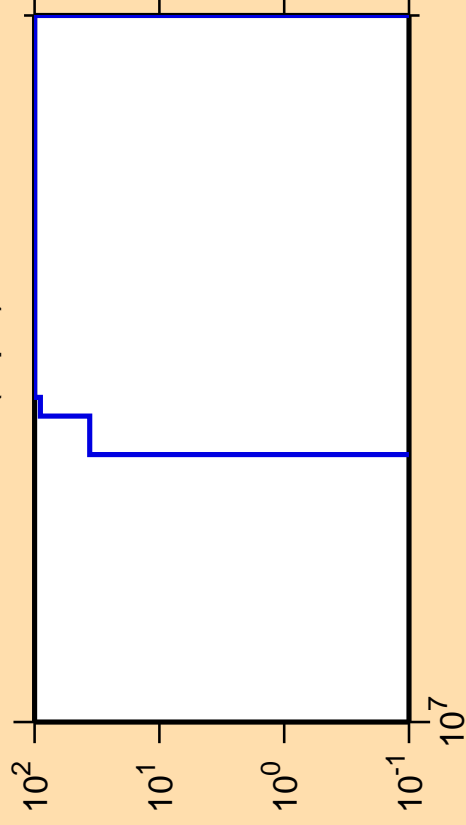
\Delta\sigma/\sigma vs. E for ^{202}\text{At}(n,pd)
