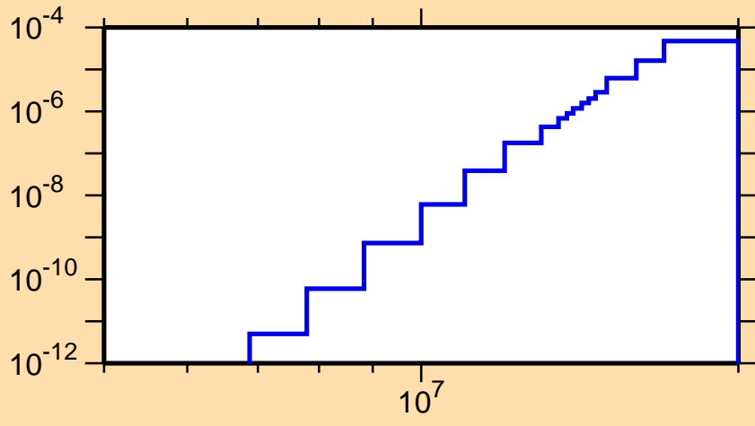
\sigma vs. E for ^{202}\text{At}(n,\text{He}3)
