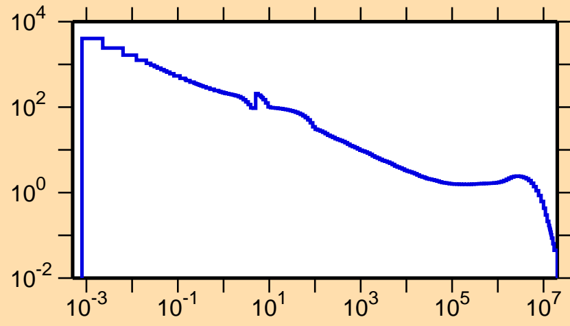
\sigma vs. E for ^{202}\text{At}(n,\gamma)
