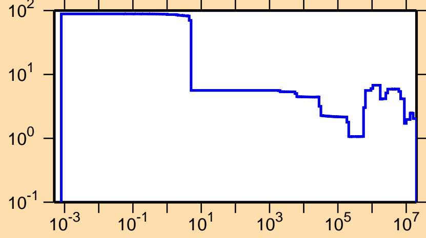
\Delta\sigma/\sigma vs. E for ^{202}\text{At}(n,\text{el.})
