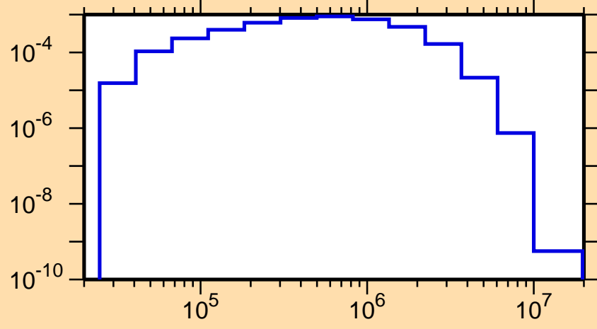
\sigma vs. E for ^{202}\text{At}(n,n_2)
