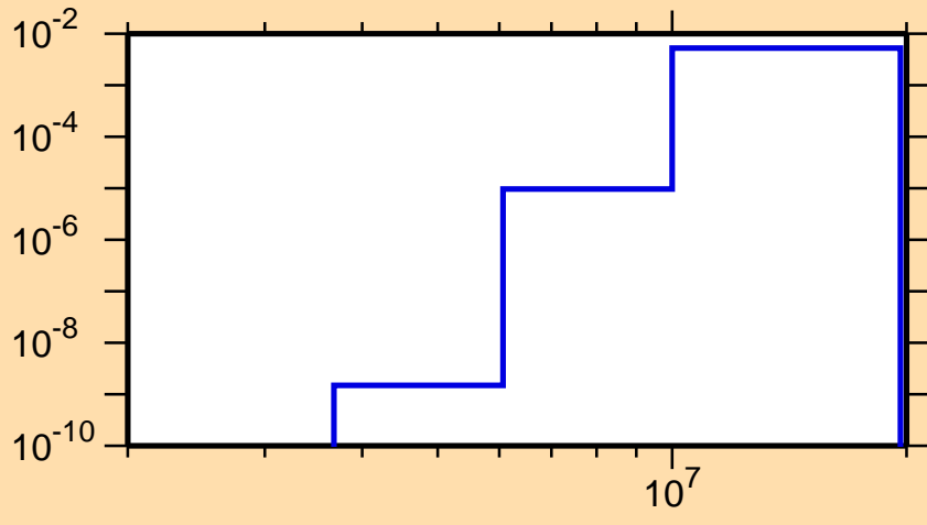
\sigma vs. E for ^{202}\text{At}(n,d)
