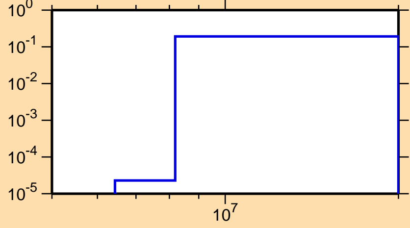
\sigma vs. E for ^{202}\text{At}(n,2n)
