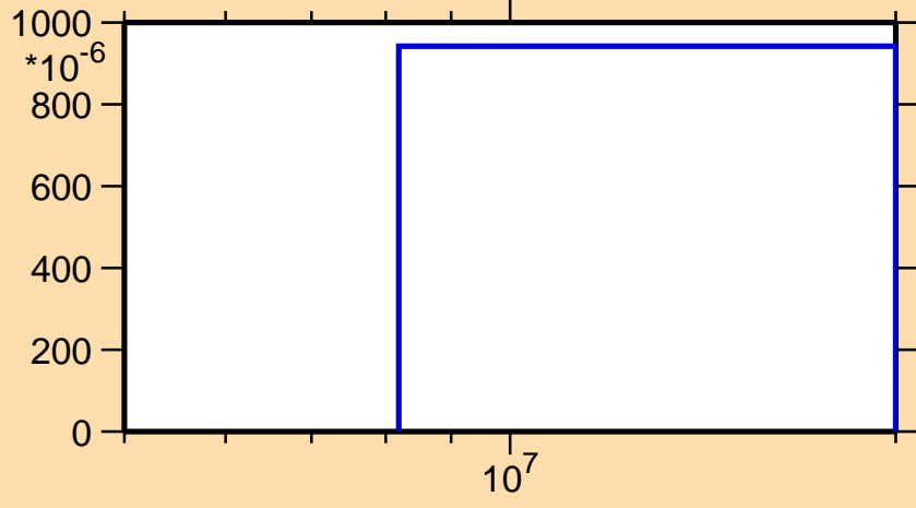
\sigma vs. E for ^{202}\text{At}(n,2n\alpha)
