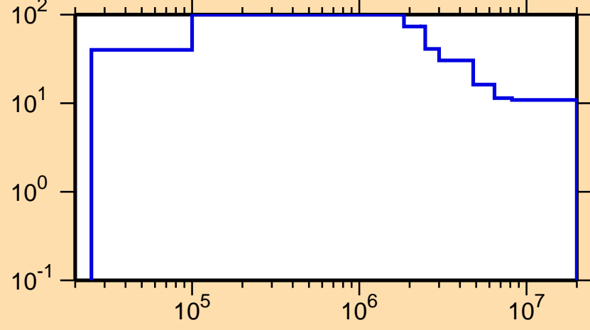
\Delta\sigma/\sigma vs. E for ^{202}\text{At}(n,n\text{cont.})
