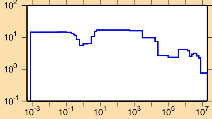
\Delta\sigma/\sigma vs. E for ^{202}\text{At}(n,\text{tot.})
