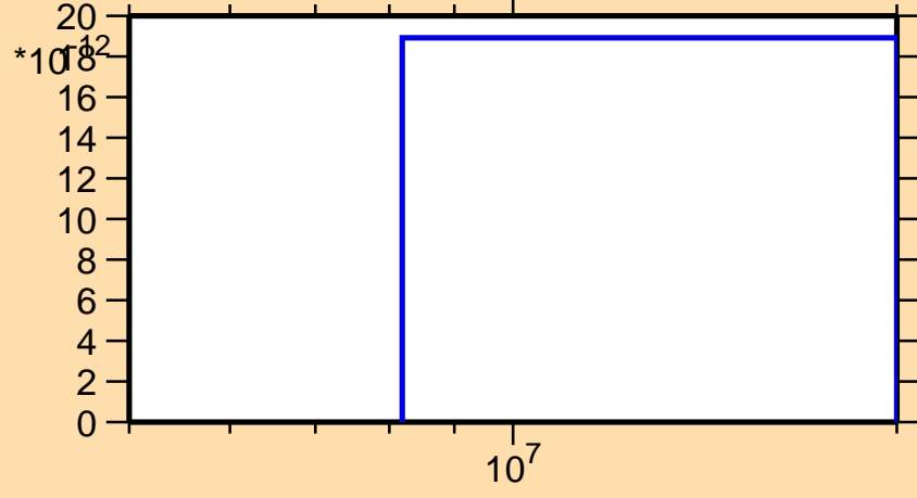
\sigma vs. E for ^{202}\text{At}(n,\text{pt})
