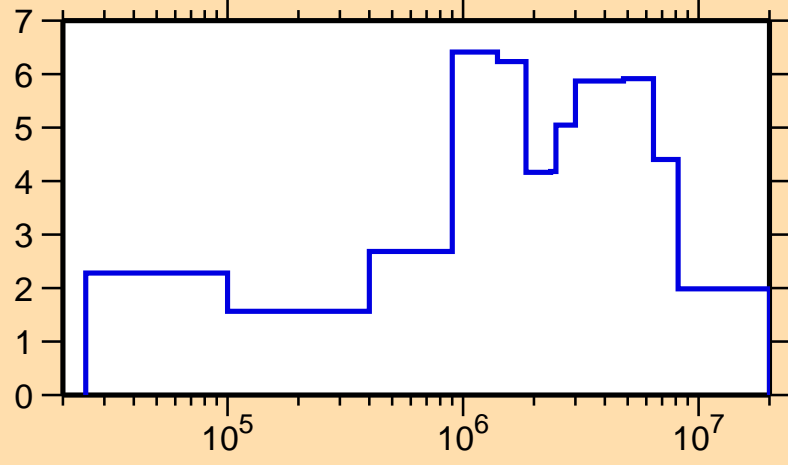
\Delta\sigma/\sigma vs. E for ^{202}\text{At}(n, el.)
