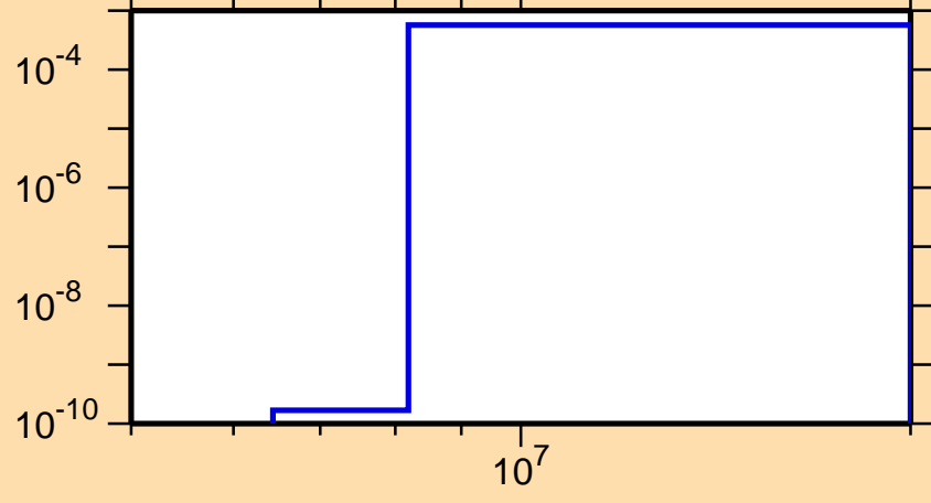
\sigma vs. E for ^{202}\text{At}(n,t)
