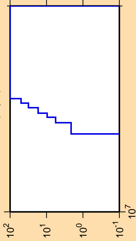
\Delta\sigma/\sigma vs. E for ^{203}\text{At}(n,pd)
