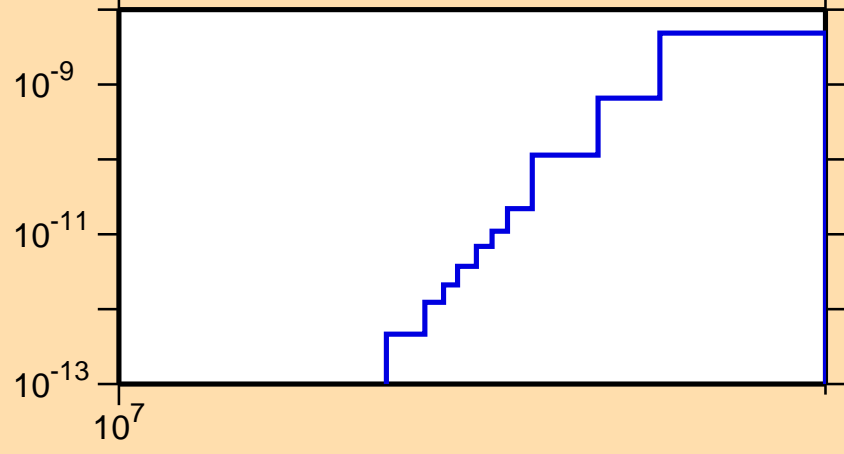
\sigma vs. E for ^{203}\text{At}(n,pd)
