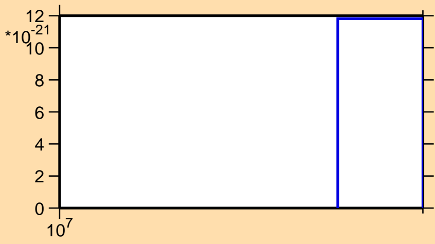
\sigma vs. E for ^{203}\text{At}(\text{mt } 42)
