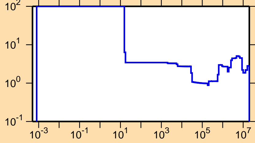
\Delta\sigma/\sigma vs. E for ^{203}\text{At}(n,\text{el.})
