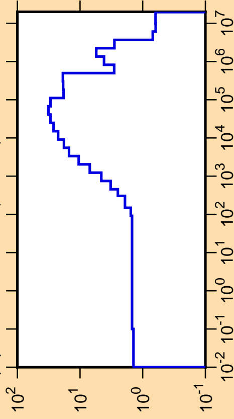
\Delta\mu/\mu vs. E for ^{203}\text{At}(\text{mt251})
