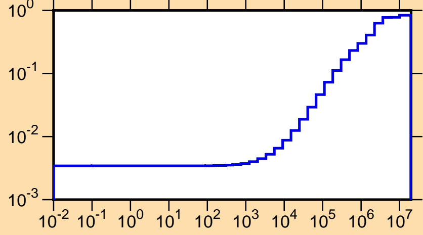
\mu vs. E for ^{203}\text{At}(\text{mt251})
