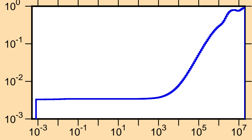
\mu vs. E for ^{204}\text{At}(\text{mt251})
