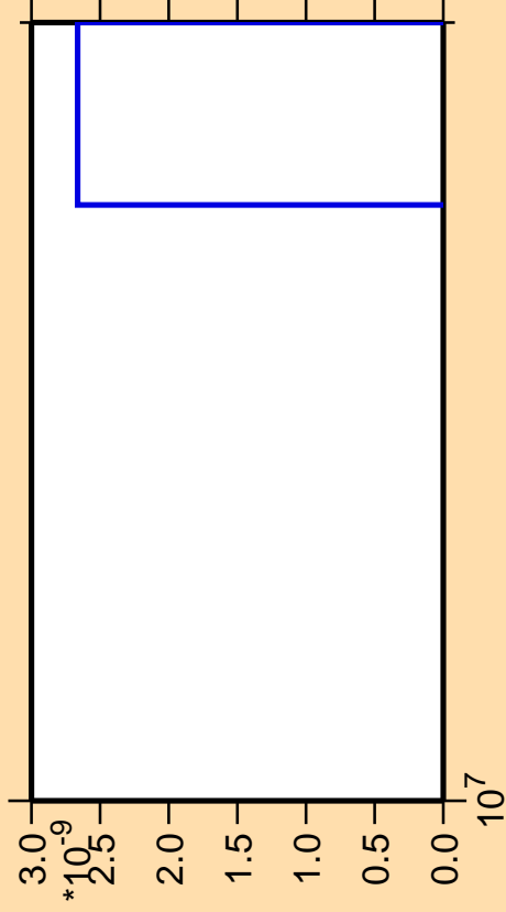
\Delta\sigma/\sigma vs. E for ^{204}\text{At}(\text{mt } 42)
