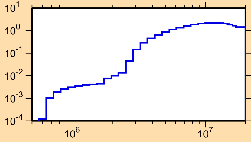
\sigma vs. E for ^{204}\text{At}(n,\text{inel.})
