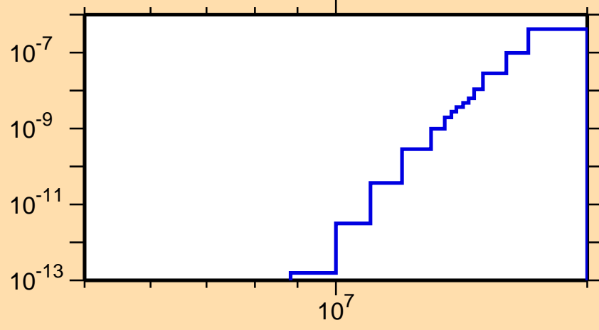
\sigma vs. E for ^{204}\text{At}(\text{mt } 45)
