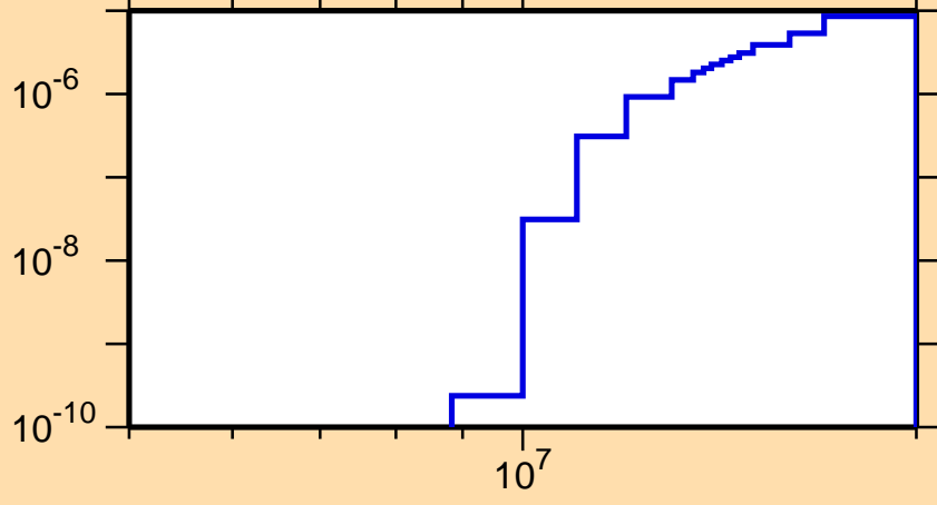
\sigma vs. E for ^{204}\text{At}(n,2n\alpha)
