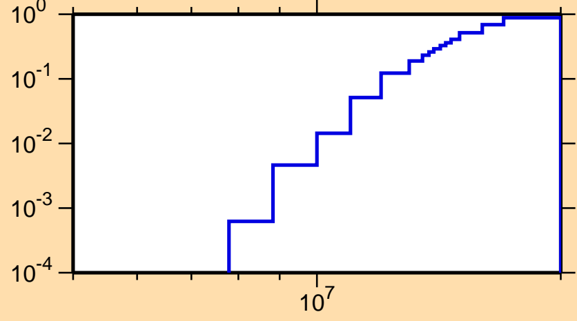
\sigma vs. E for ^{204}\text{At}(n,2n)
