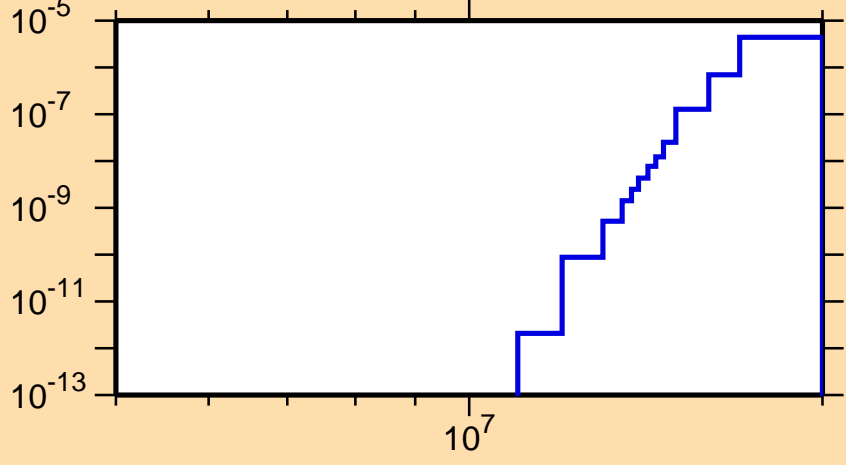
\sigma vs. E for ^{204}\text{At}(n,\text{nd})
