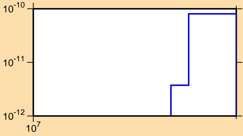
\sigma vs. E for ^{204}\text{At}(\text{mt } 34)
