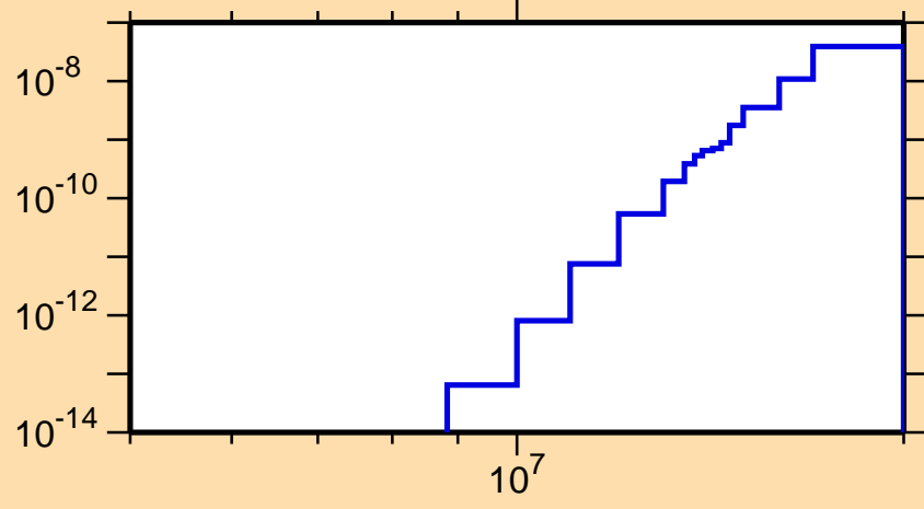
\sigma vs. E for ^{204}\text{At}(\text{mt117})
