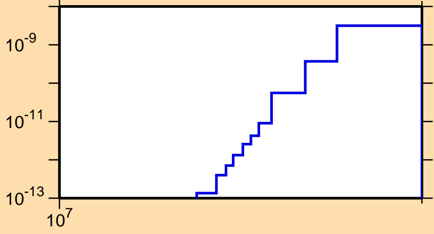
\sigma vs. E for ^{204}\text{At}(n,pd)
