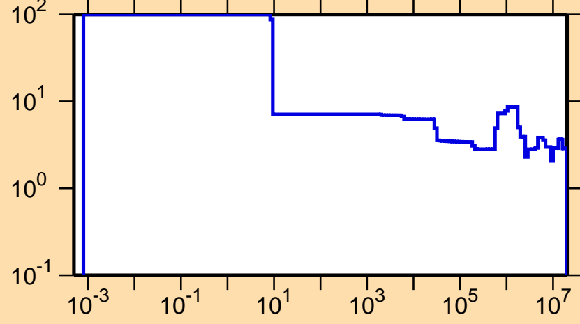
\Delta\sigma/\sigma vs. E for ^{204}\text{At}(n,\text{el.})
