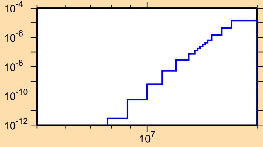
\sigma vs. E for ^{204}\text{At}(n,\text{He}3)
