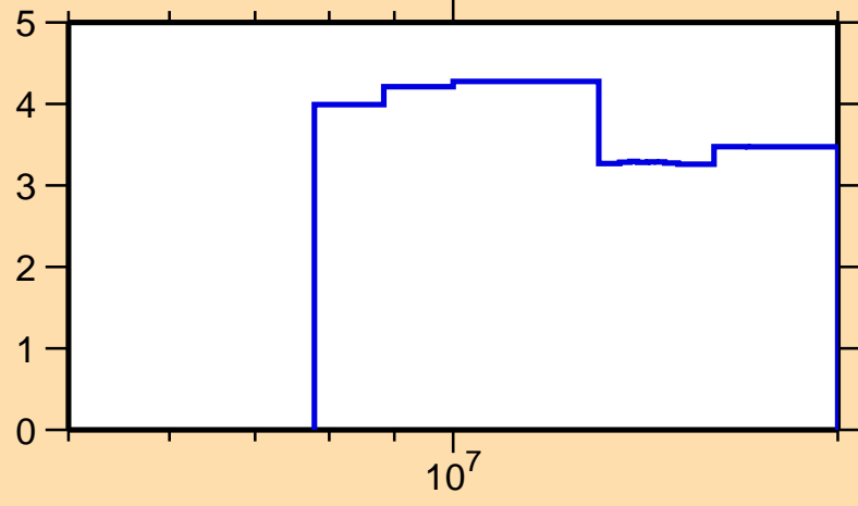
\Delta\sigma/\sigma vs. E for ^{204}\text{At}(n,\text{nonel.})
