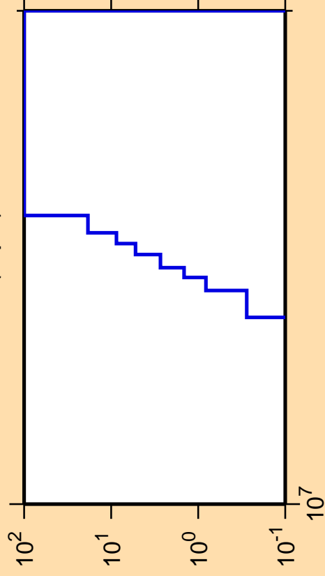
\Delta\sigma/\sigma vs. E for ^{204}\text{At}(n,pd)
