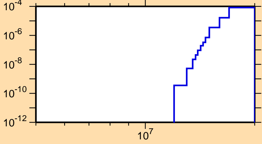
\sigma vs. E for ^{204}\text{At}(n,2np)
