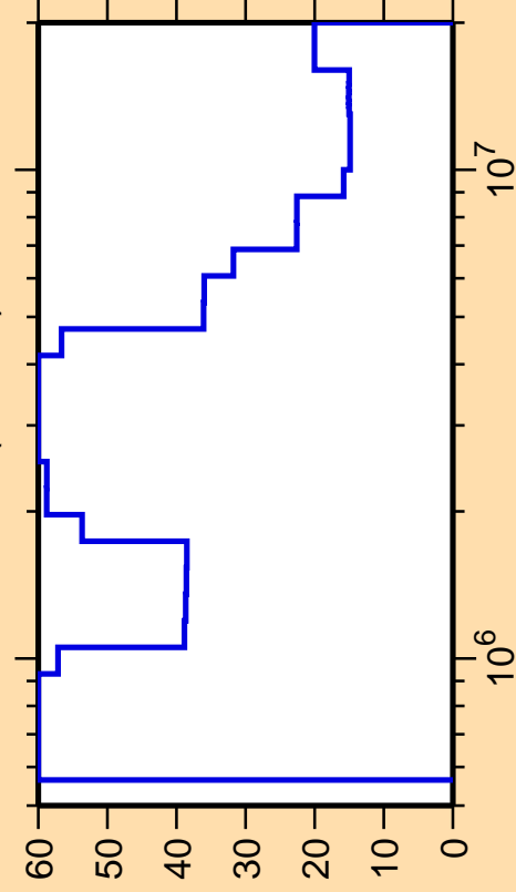
\Delta\sigma/\sigma vs. E for ^{204}\text{At}(n,\text{inel.})
