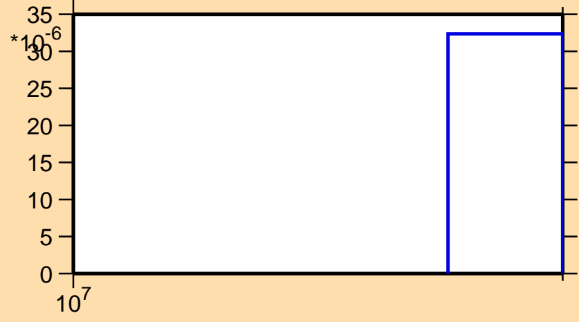
\sigma vs. E for ^{204}\text{At}(n,3n)
