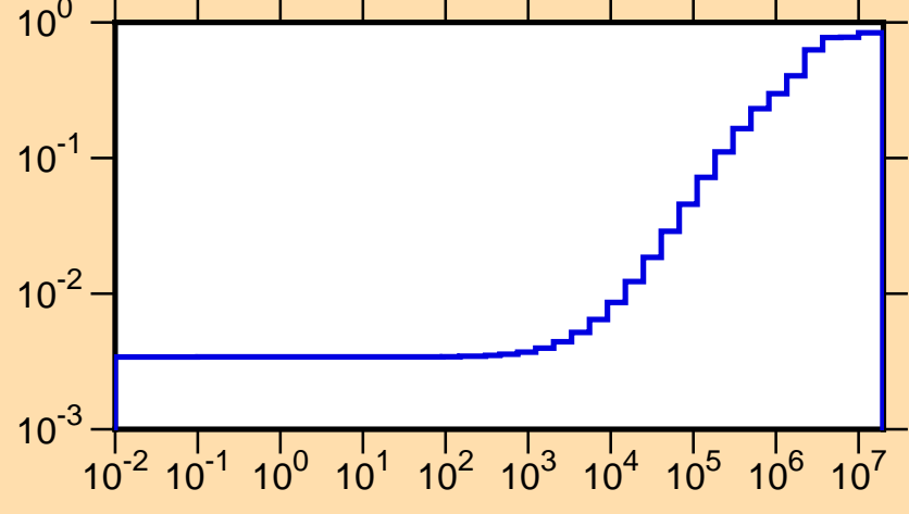
\mu vs. E for ^{204}\text{At}(\text{mt251})
