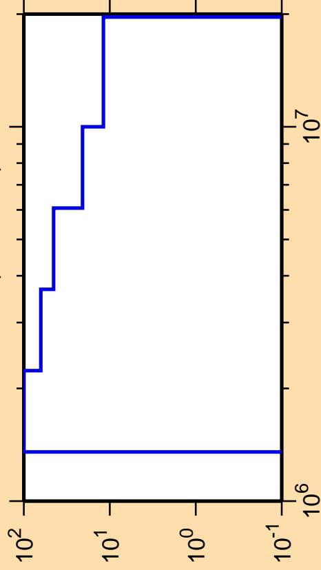
\Delta\sigma/\sigma vs. E for ^{204}\text{At}(n,\text{ncont.})
