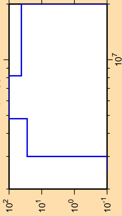
\Delta\sigma/\sigma vs. E for ^{204}\text{At}(n,np)
