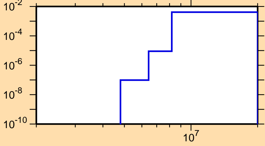
\sigma vs. E for ^{204}\text{At}(n,np)
