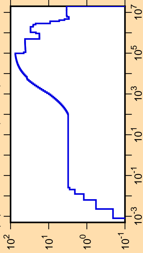
\Delta\mu/\mu vs. E for ^{205}\text{At}(\text{mt251})
