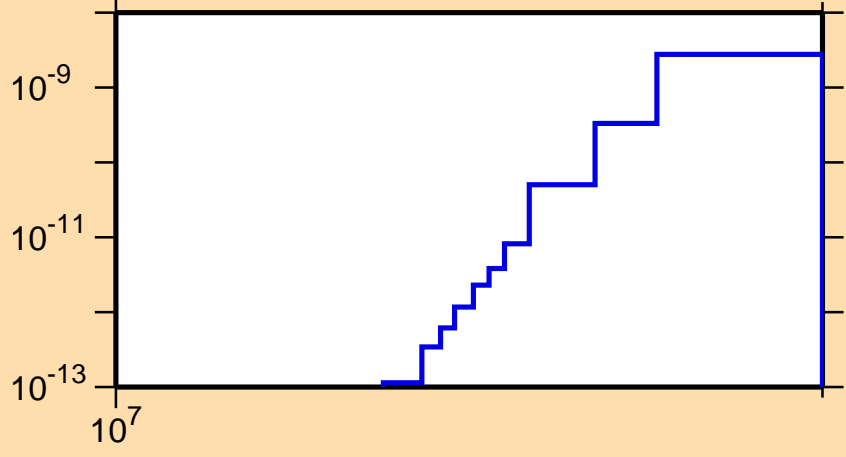
\sigma vs. E for ^{205}\text{At}(n,pd)
