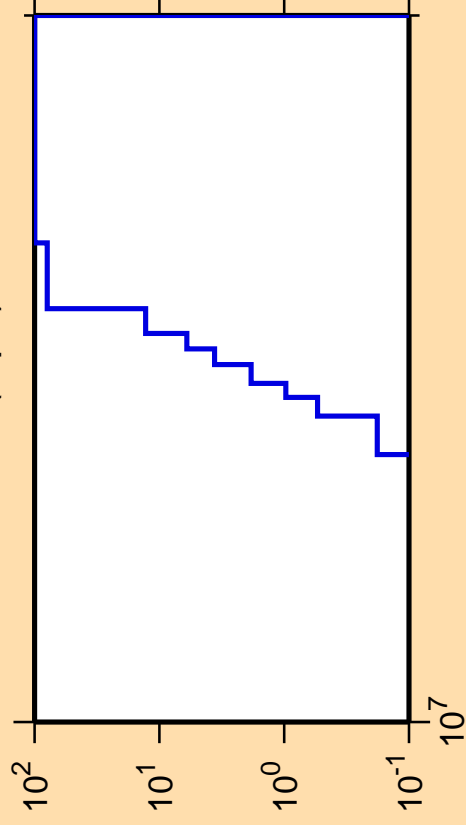
\Delta\sigma/\sigma vs. E for ^{205}\text{At}(n,pd)
