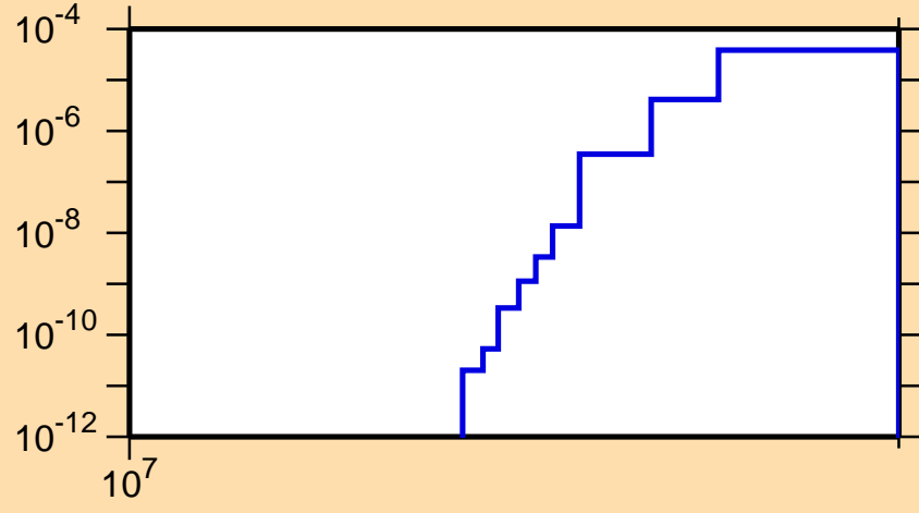
\sigma vs. E for ^{205}\text{At}(n,2np)
