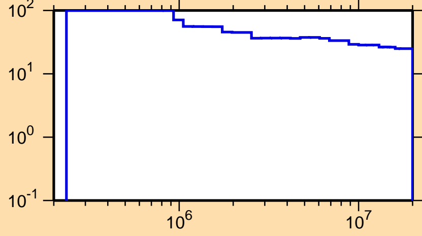
\Delta\sigma/\sigma vs. E for ^{205}\text{At}(n,n_1)
