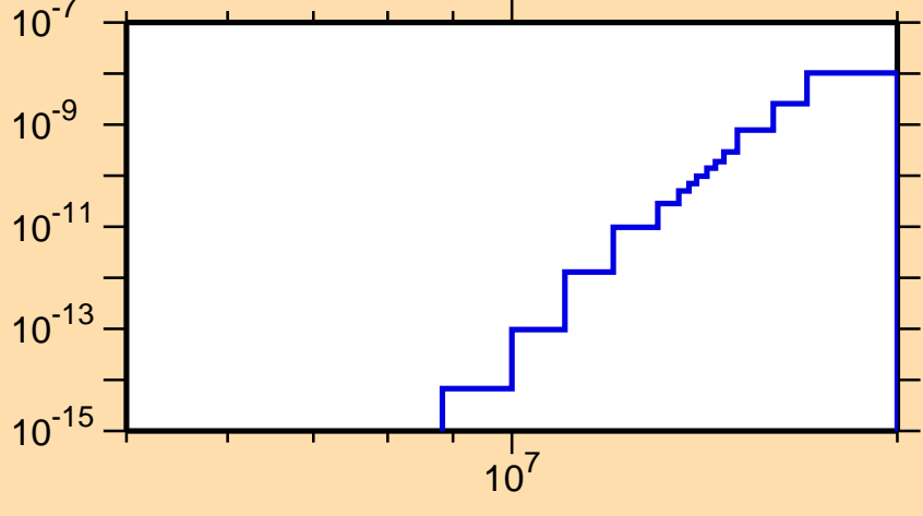
\sigma vs. E for ^{205}\text{At}(\text{mt } 45)
