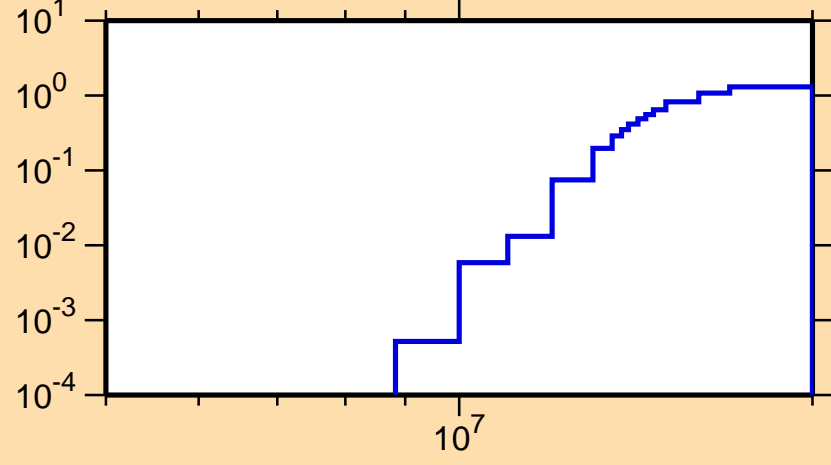
\sigma vs. E for ^{205}\text{At}(n,2n)
