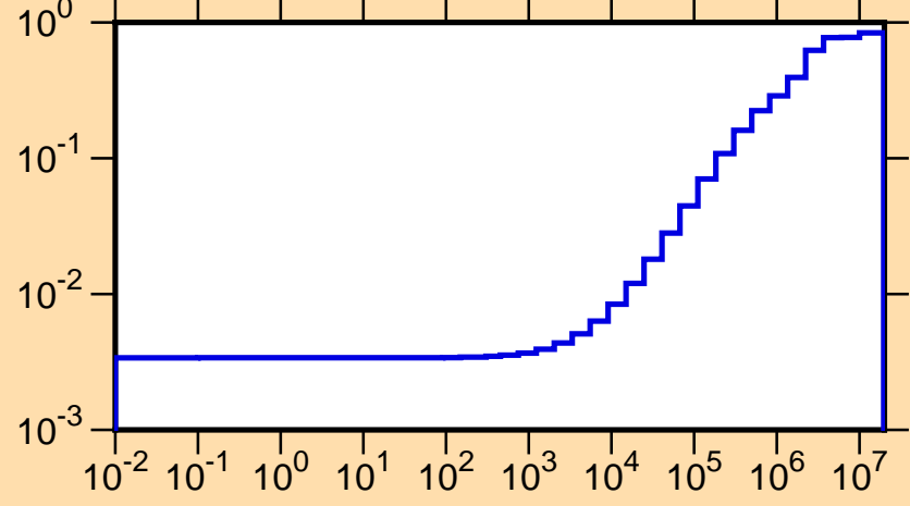
\mu vs. E for ^{205}\text{At}(\text{mt251})
