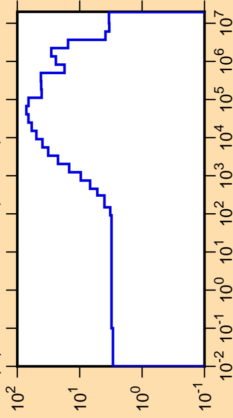
\Delta\mu/\mu vs. E for ^{205}\text{At}(\text{mt251})
