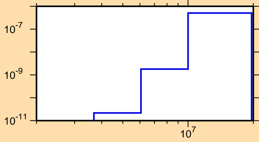
\sigma vs. E for ^{205}\text{At}(n,p\alpha)
