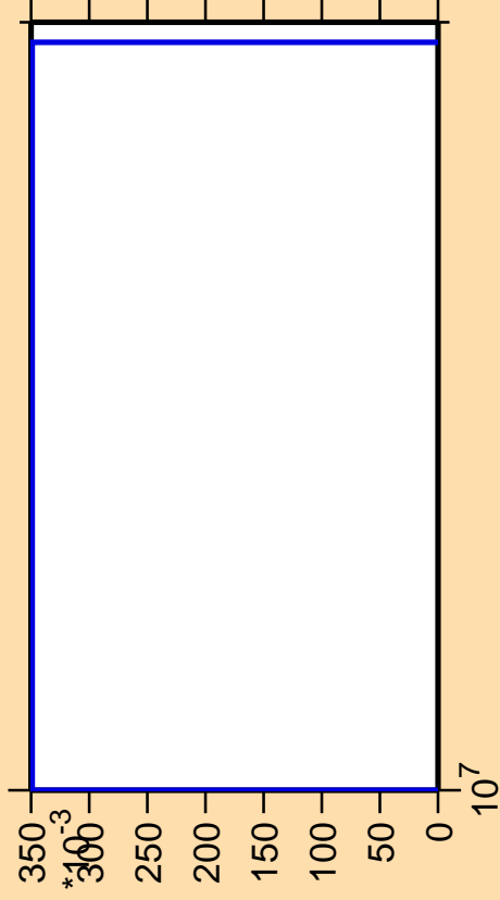
\Delta\sigma/\sigma vs. E for ^{205}\text{At}(n,\text{pt})
