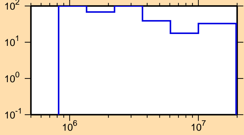
\Delta\sigma/\sigma vs. E for ^{205}\text{At}(n,n\text{cont.})
