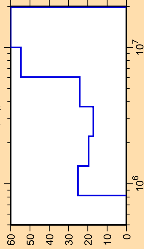
\Delta\sigma/\sigma vs. E for ^{205}\text{At}(n,\gamma)
