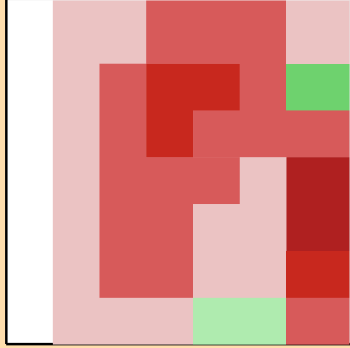
\Delta\sigma/\sigma vs. E for ^{205}\text{At}(n,n\text{cont.})
