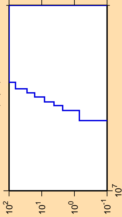
\Delta\sigma/\sigma vs. E for ^{206}\text{At}(n,pd)
