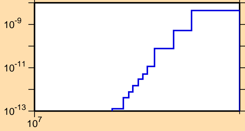
\sigma vs. E for ^{206}\text{At}(n,pd)
