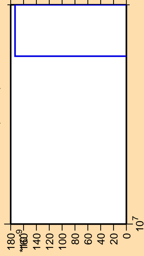
\Delta\sigma/\sigma vs. E for ^{206}\text{At}(\text{mt } 42)
