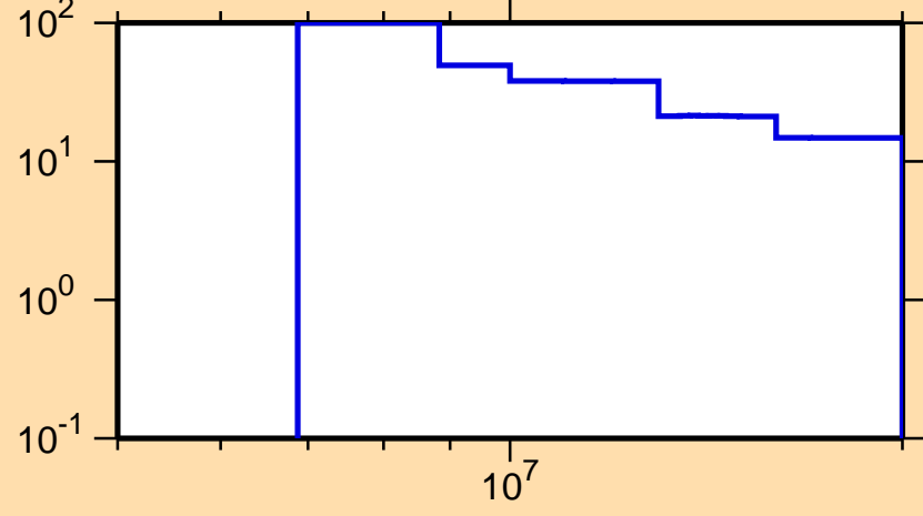
\Delta\sigma/\sigma vs. E for ^{206}\text{At}(n,2n)
