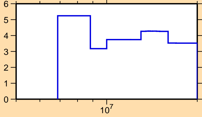
\Delta\sigma/\sigma vs. E for ^{206}\text{At}(n,\text{tot.})
