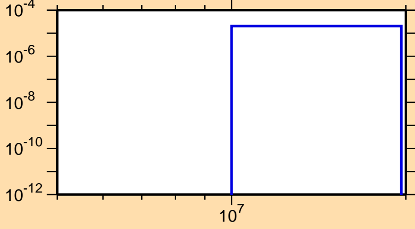
\sigma vs. E for ^{206}\text{At}(n,2np)
