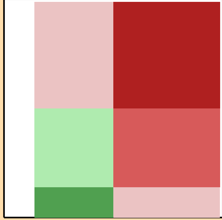
\Delta\sigma/\sigma vs. E for ^{206}\text{At}(n,2n)
