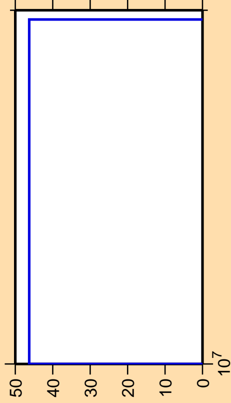
\Delta\sigma/\sigma vs. E for ^{206}\text{At}(n,\text{pt})
