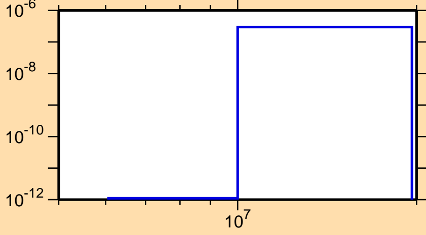
\sigma vs. E for ^{206}\text{At}(n,\text{He}3)
