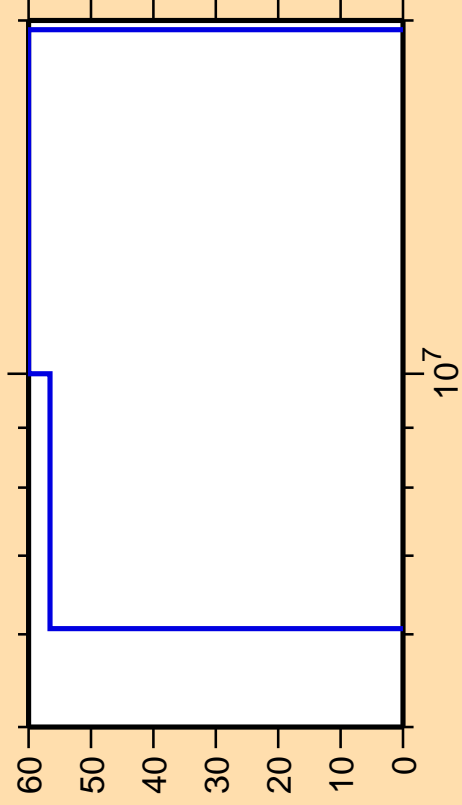
\Delta\sigma/\sigma vs. E for ^{206}\text{At}(n,\gamma)
