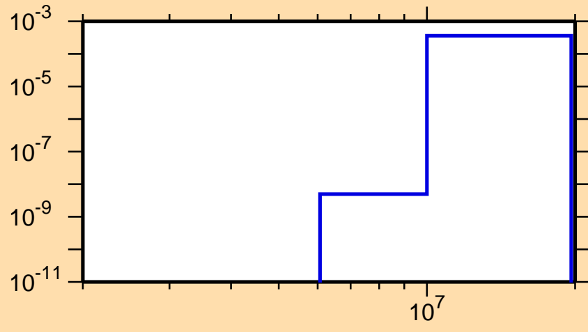
\sigma vs. E for ^{206}\text{At}(n,t)
