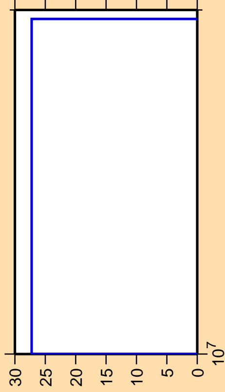
\Delta\sigma/\sigma vs. E for ^{206}\text{At}(\text{mt } 34)
