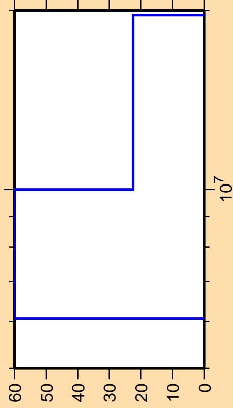
\Delta\sigma/\sigma vs. E for ^{206}\text{At}(n,2n)
