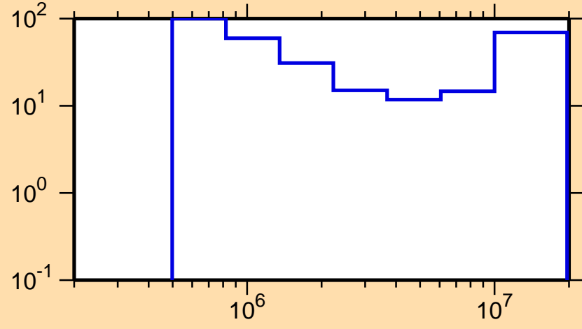
\Delta\sigma/\sigma vs. E for ^{206}\text{At}(n,n\text{cont.})
