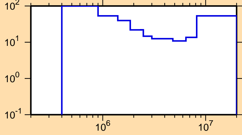
\Delta\sigma/\sigma vs. E for ^{206}\text{At}(n,ncont.)
