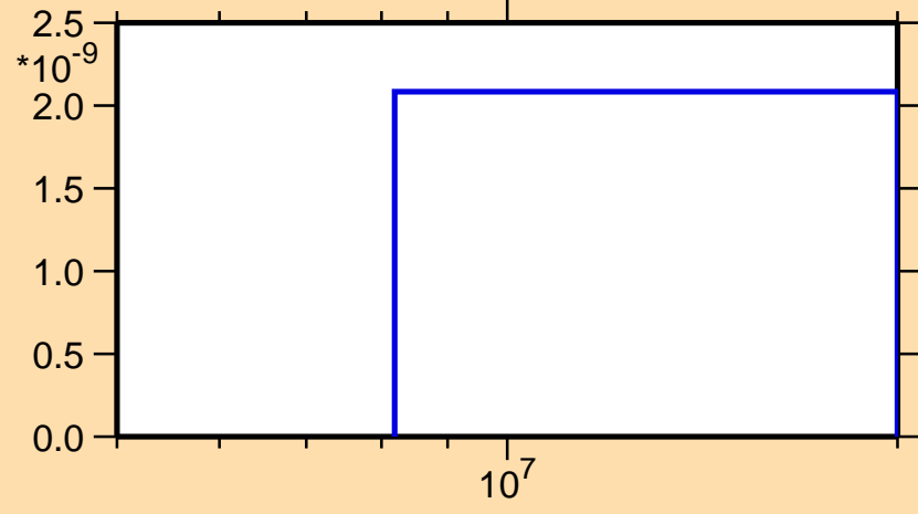
\sigma vs. E for ^{206}\text{At}(n,nt)
