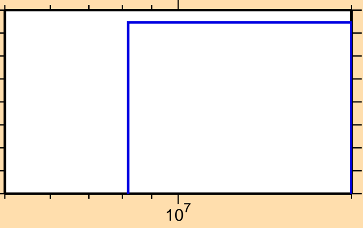
\sigma vs. E for ^{206}\text{At}(n,3n)
