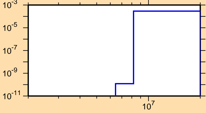
\sigma vs. E for ^{206}\text{At}(n,t)
