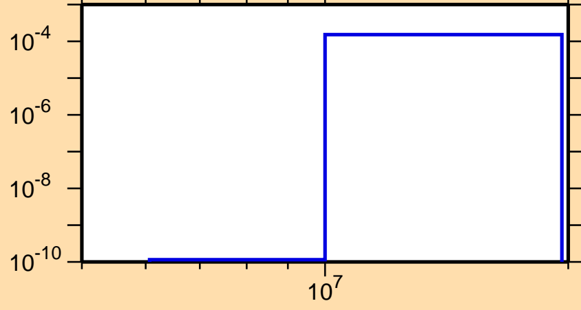
\sigma vs. E for ^{207}\text{At}(n,t)
