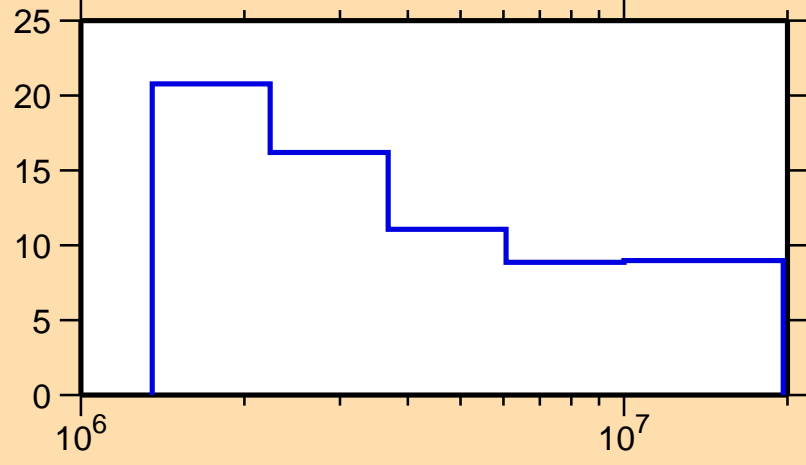
\Delta\sigma/\sigma vs. E for ^{207}\text{At}(n,n\text{onel.})
