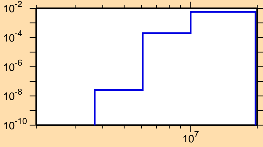
\sigma vs. E for ^{207}\text{At}(n,np)
