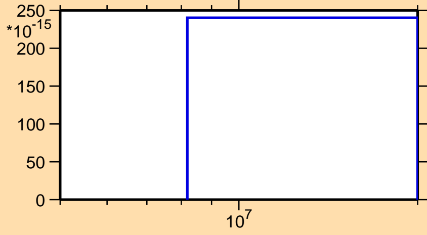
\sigma vs. E for ^{207}\text{At}(n,\text{pt})
