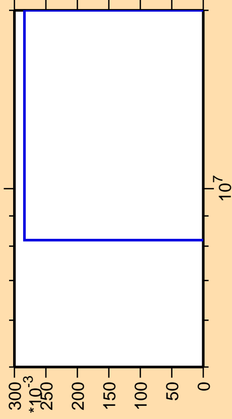
\Delta\sigma/\sigma vs. E for ^{207}\text{At}(n,\text{pt})
