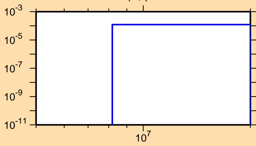
\sigma vs. E for ^{207}\text{At}(n,t)
