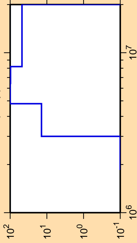
\Delta\sigma/\sigma vs. E for ^{207}\text{At}(n,np)
