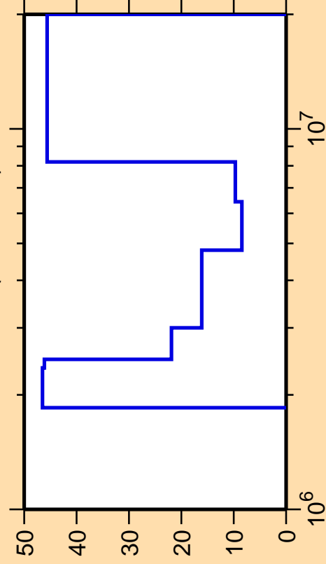
\Delta\sigma/\sigma vs. E for ^{207}\text{At}(n,\text{ncont.})
