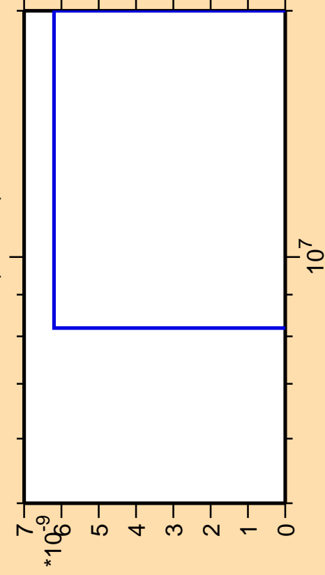
\Delta\sigma/\sigma vs. E for ^{207}\text{At}(\text{mt } 42)
