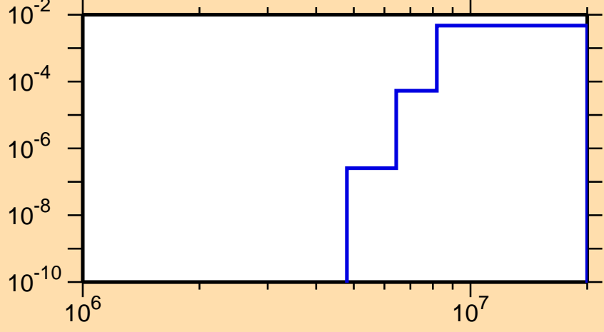
\sigma vs. E for ^{207}\text{At}(n,np)
