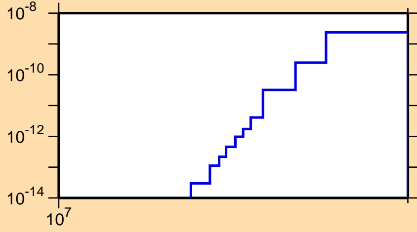
\sigma vs. E for ^{208}\text{At}(n,pd)
