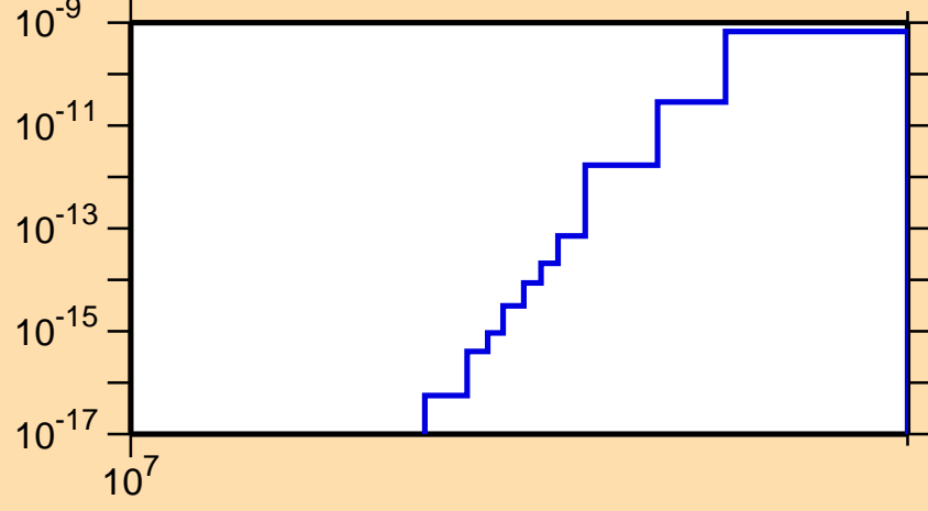
\sigma vs. E for ^{208}\text{At}(n,pt)
