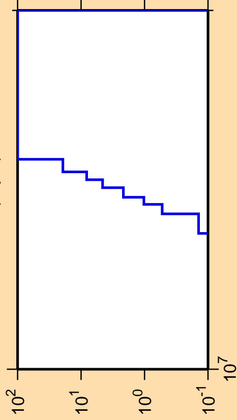
\Delta\sigma/\sigma vs. E for ^{208}\text{At}(n,pd)
