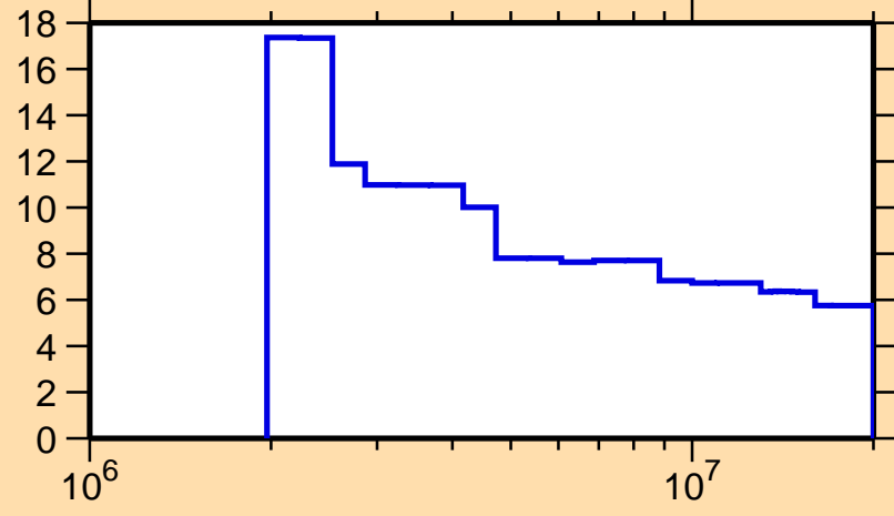
\Delta\sigma/\sigma vs. E for ^{209}\text{At}(n,n\text{onel.})
