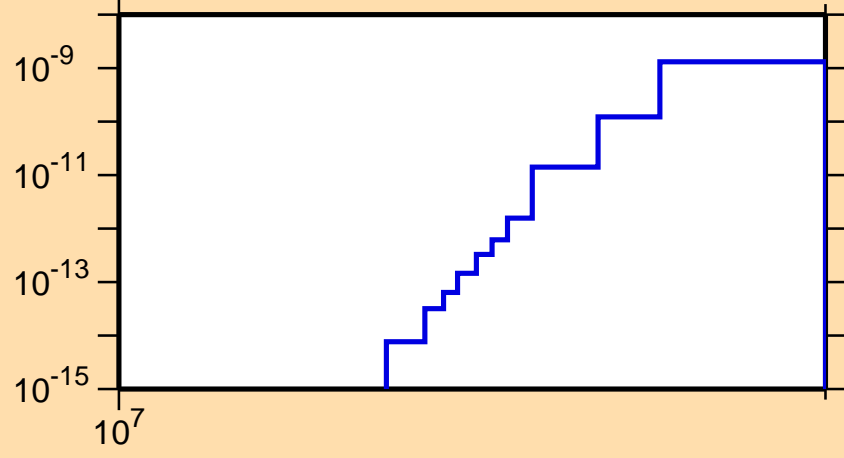
\sigma vs. E for ^{209}\text{At}(n,pd)
