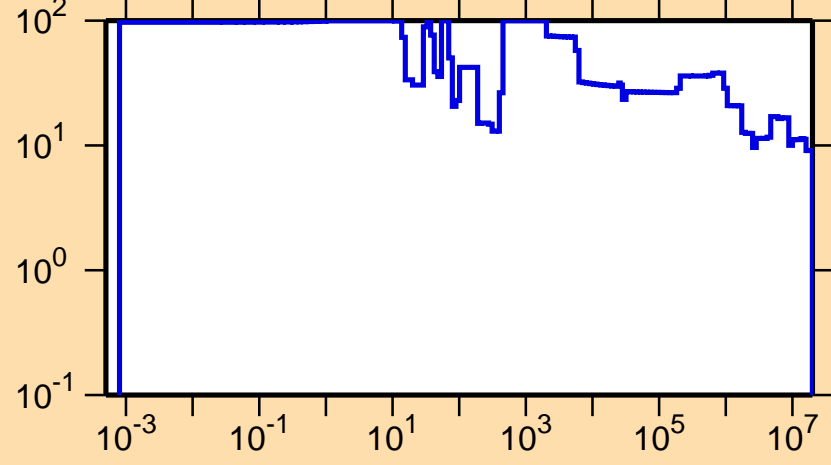
\Delta\sigma/\sigma vs. E for ^{209}\text{At}(n,\text{el.})
