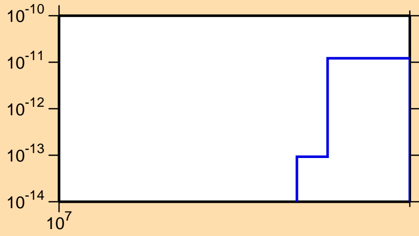
\sigma vs. E for ^{209}\text{At}(\text{mt } 34)
