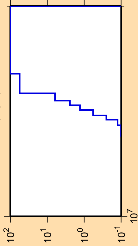
\Delta\sigma/\sigma vs. E for ^{209}\text{At}(n,pd)
