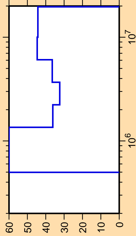
\Delta\sigma/\sigma vs. E for ^{209}\text{At}(n,n_3)
