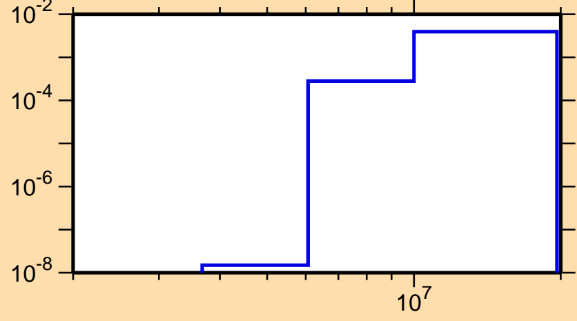
\sigma vs. E for ^{209}\text{At}(n,np)
