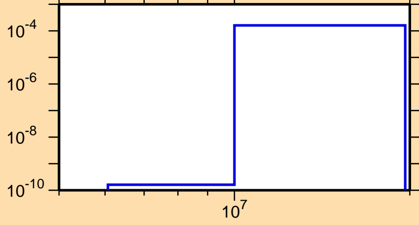
\sigma vs. E for ^{209}\text{At}(n,t)
