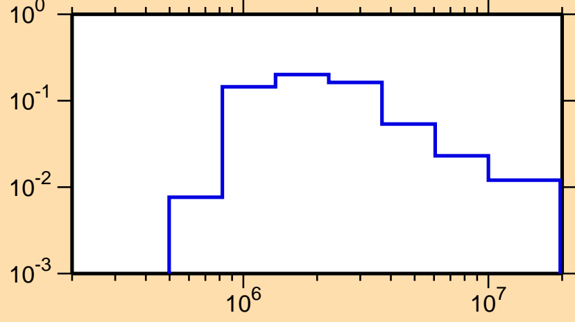
\sigma vs. E for ^{209}\text{At}(n,n_3)
