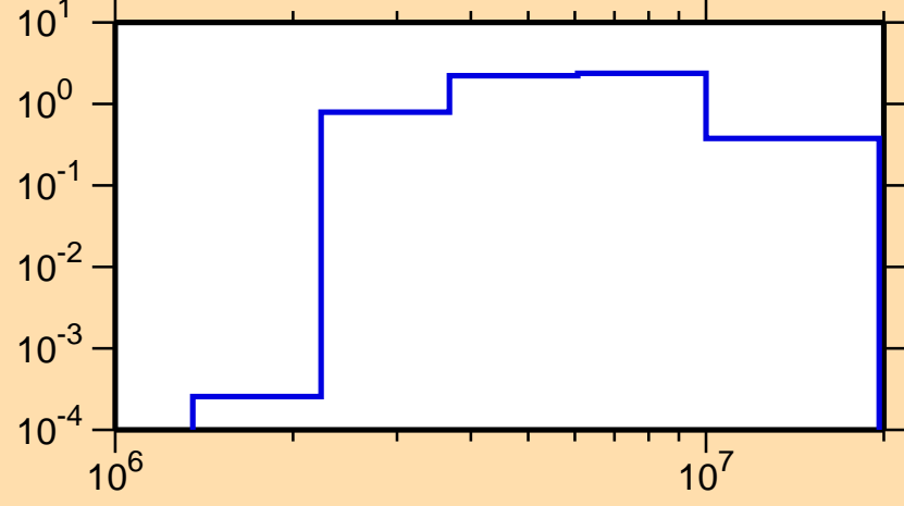
\sigma vs. E for ^{209}\text{At}(n,n\text{cont.})
