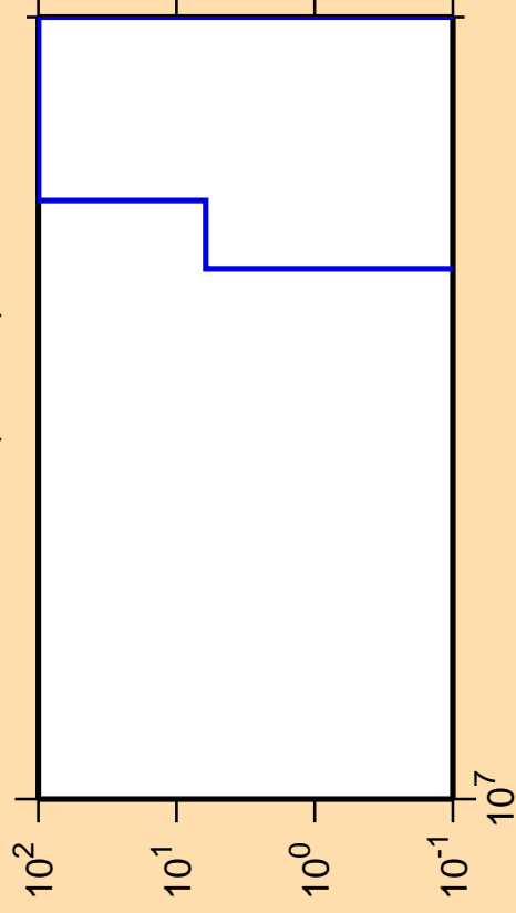
\Delta\sigma/\sigma vs. E for ^{210}\text{At} (mt 34)
