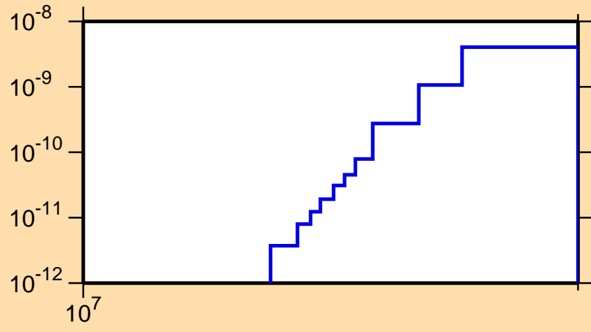
\sigma vs. E for ^{210}\text{At}(\text{mt117})
