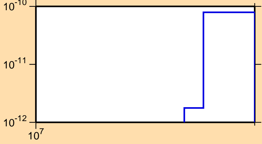
\sigma vs. E for ^{210}\text{At} (mt 34)
