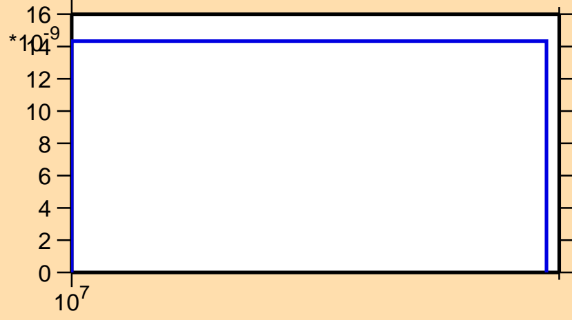
\sigma vs. E for ^{210}\text{At}(n,nt)
