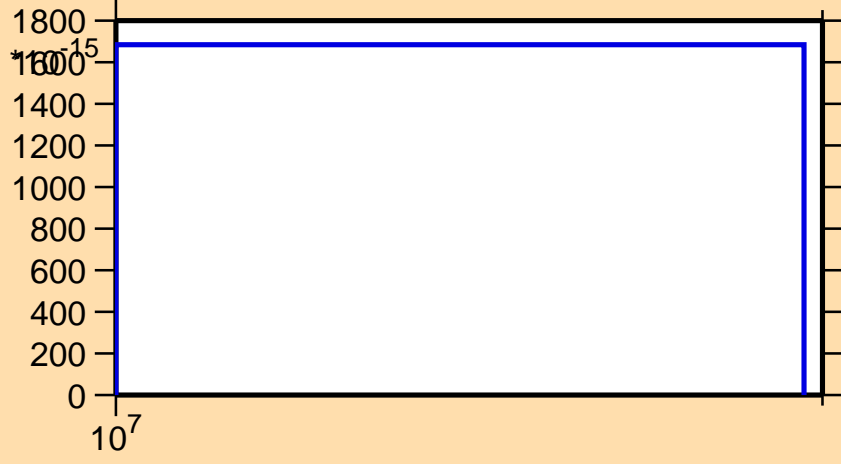
\sigma vs. E for ^{210}\text{At}(n,\text{pt})
