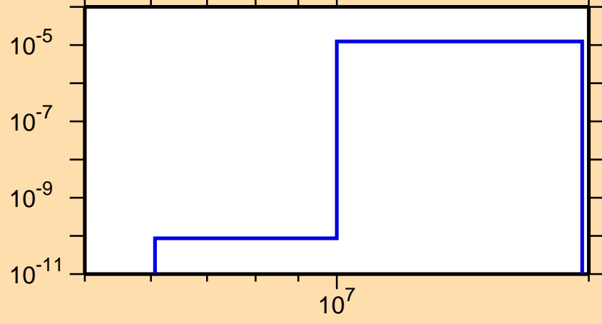
\sigma vs. E for ^{210}\text{At}(n,2n\alpha)
