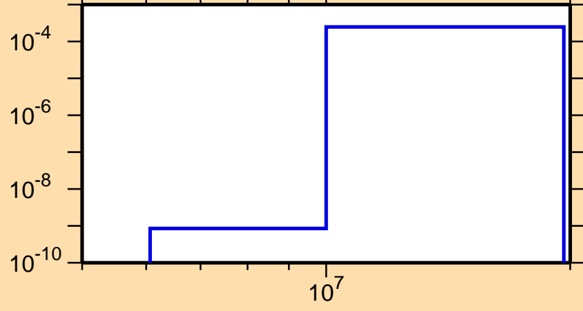
\sigma vs. E for ^{211}\text{At}(n,t)
