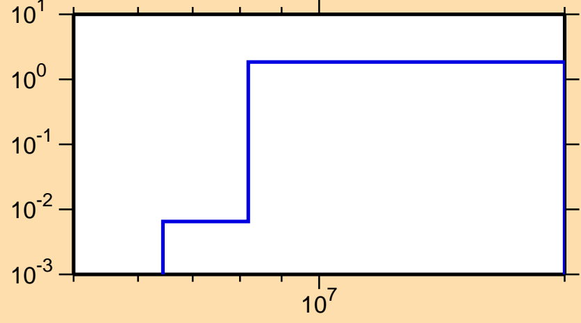
\sigma vs. E for ^{211}\text{At}(n,2n)
