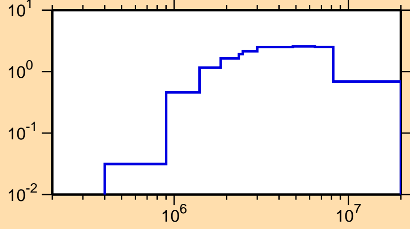
\sigma vs. E for ^{211}\text{At}(n,\text{inel.})
