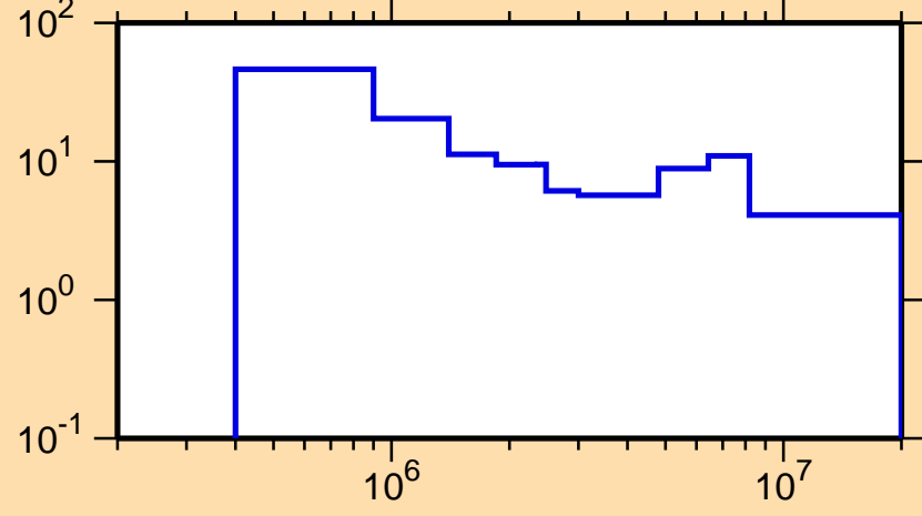
\Delta\sigma/\sigma vs. E for ^{211}\text{At}(n,\text{tot.})
