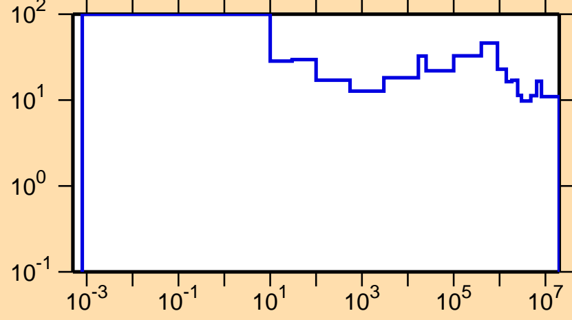
\Delta\sigma/\sigma vs. E for ^{211}\text{At}(n,\text{el.})
