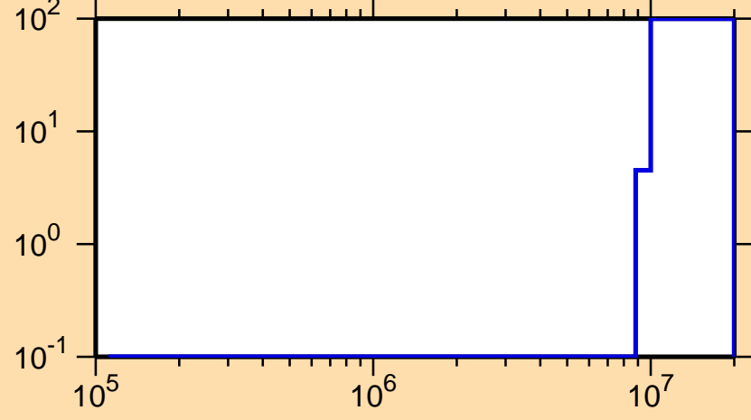
\Delta\sigma/\sigma vs. E for ^{218}\text{At}(n,f)
