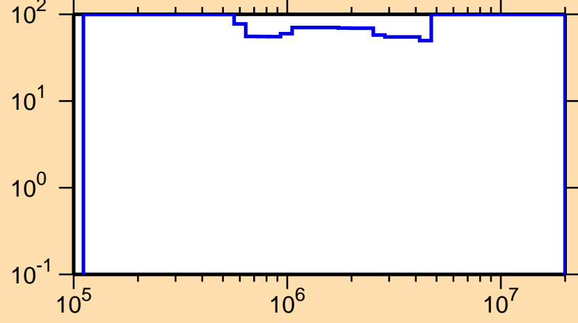
\Delta\sigma/\sigma vs. E for ^{218}\text{At}(n,n\text{cont.})
